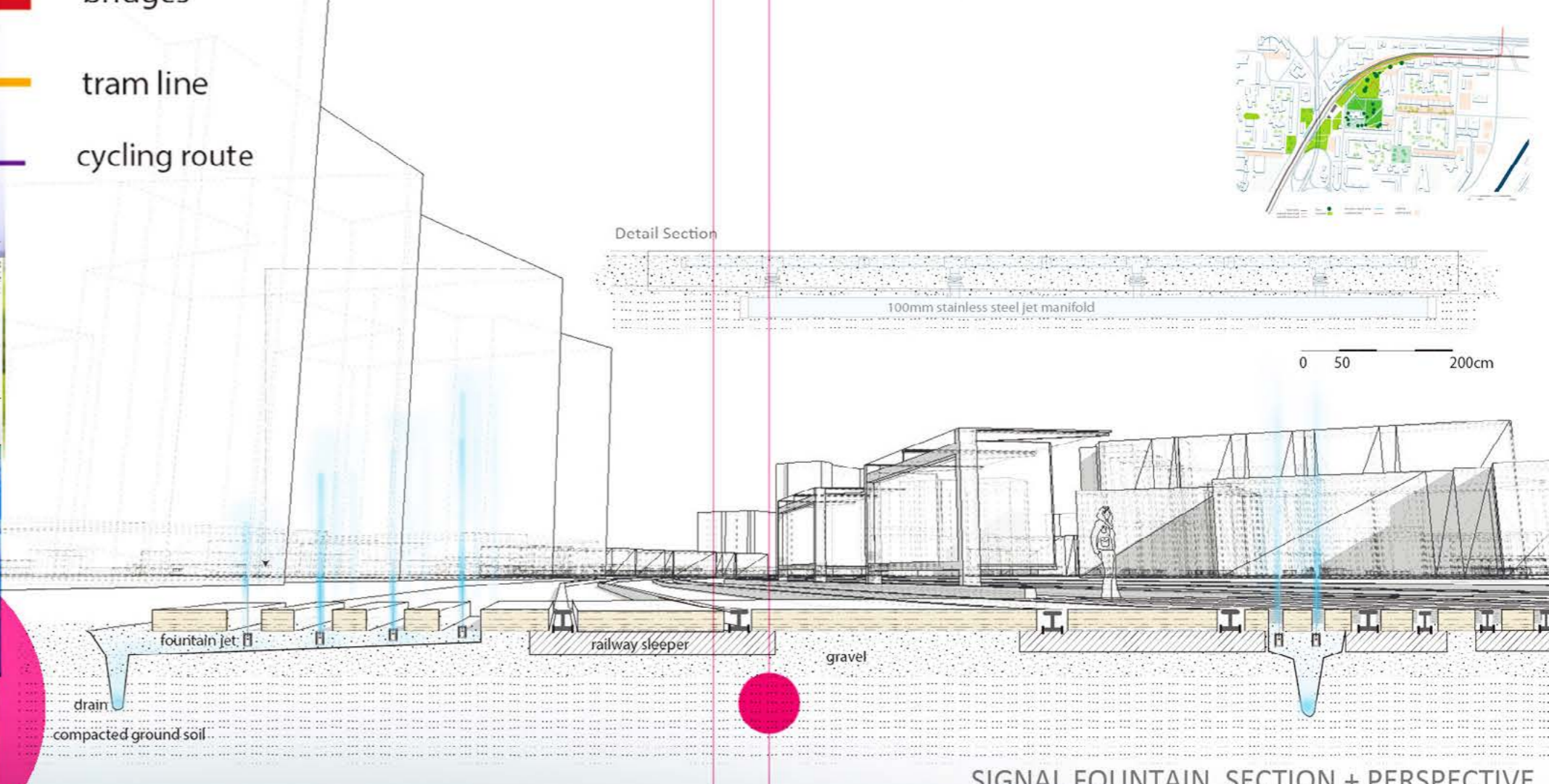
SIGNAL FOUNTAIN SECTION + PERSPECTIVE
