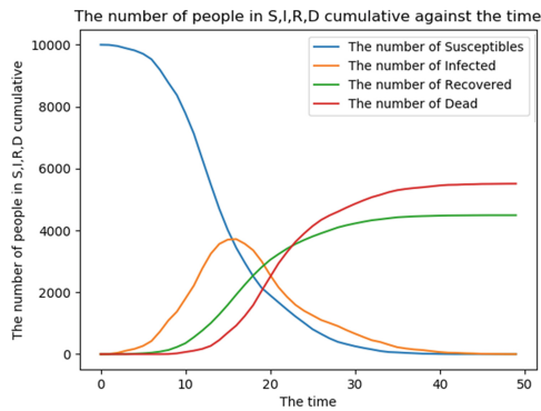
Fig. 1. Graph of the number of people in Susceptible, Infected, Recovered, Dead sub-populations cumulative against the time with no lockdown.
