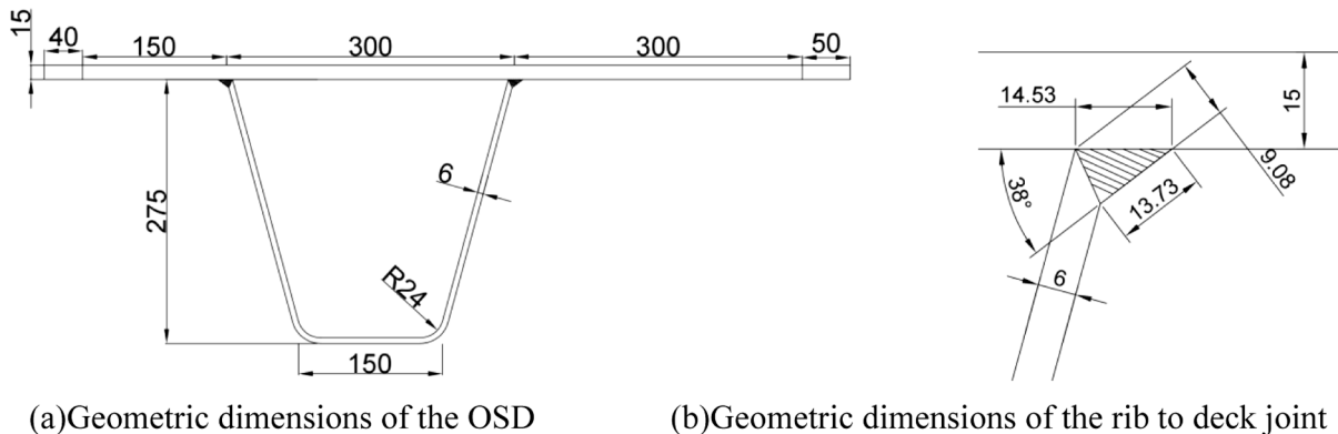
Fig. 5. Geometric dimension of the specimen [18]. (a)Geometric dimensions of the OSD (b)Geometric dimensions of the rib to deck joint.
