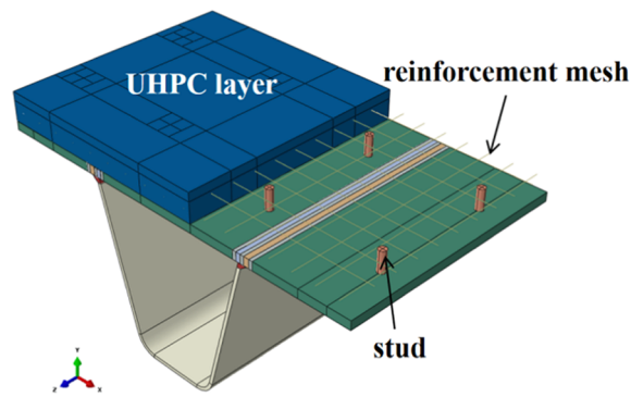
Fig. 3. conventional overall reinforcement method.
