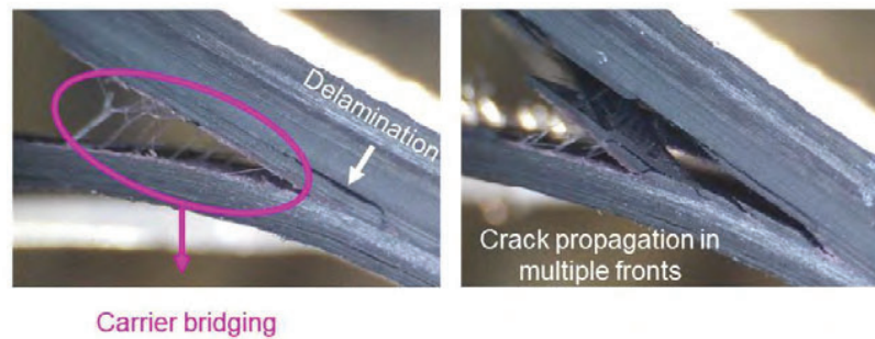
Figure 4: (a) First crack deflection to the co-cured toughening layer and (b) further deflection to the -45-degree layer of specimen Araldite [90/45/-45/AF163-2k/0] s .
