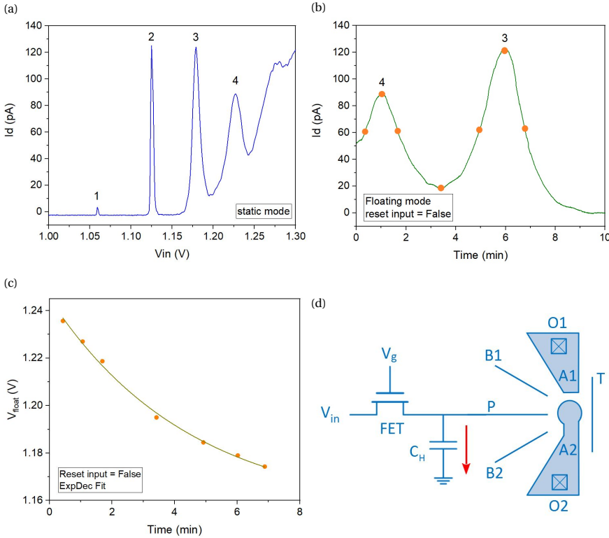
Figure 5.6: Leakage rate measurement of device A without reset input V_{in} . (a) A few Coulomb peaks measured in the static mode as reference. (b) Current through the quantum dot as function of time after floating its plunger gate. A few points (orange dots) are selected to relate the current level to the voltage on the plunger gate. (c) Voltage decay on the floating node fitted by an exponential function. (d) An indication of the main leakage path.
