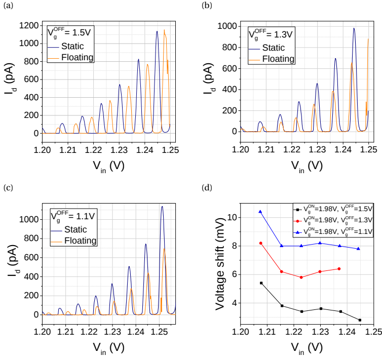
Figure 5.3: Static (blue) and floating (orange) mode Coulomb blockade peaks of device B with V_g^{ON} = 1.98V and (a) V_g^{OFF} = 1.5V , (b) V_g^{OFF} = 1.3V and (c) V_g^{OFF} = 1.1V . The peak shifts are summarized in (d) as a function of the input voltage in the static mode.
