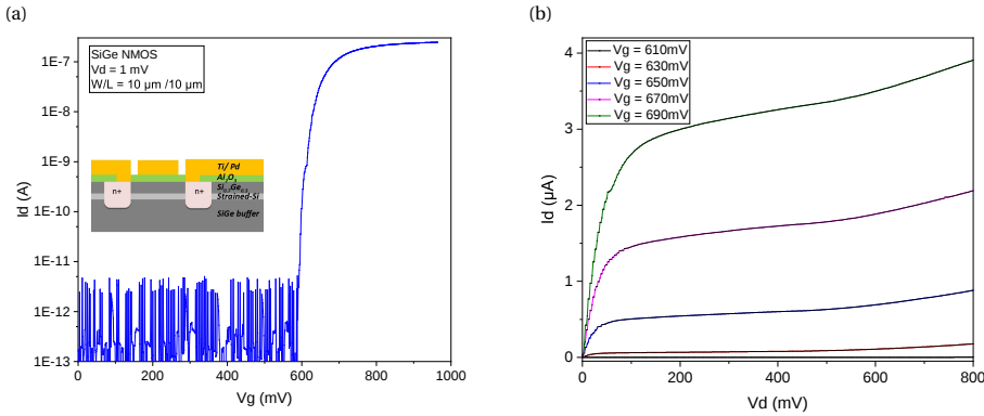
Figure 4.4: Transfer and output curve of FET1
