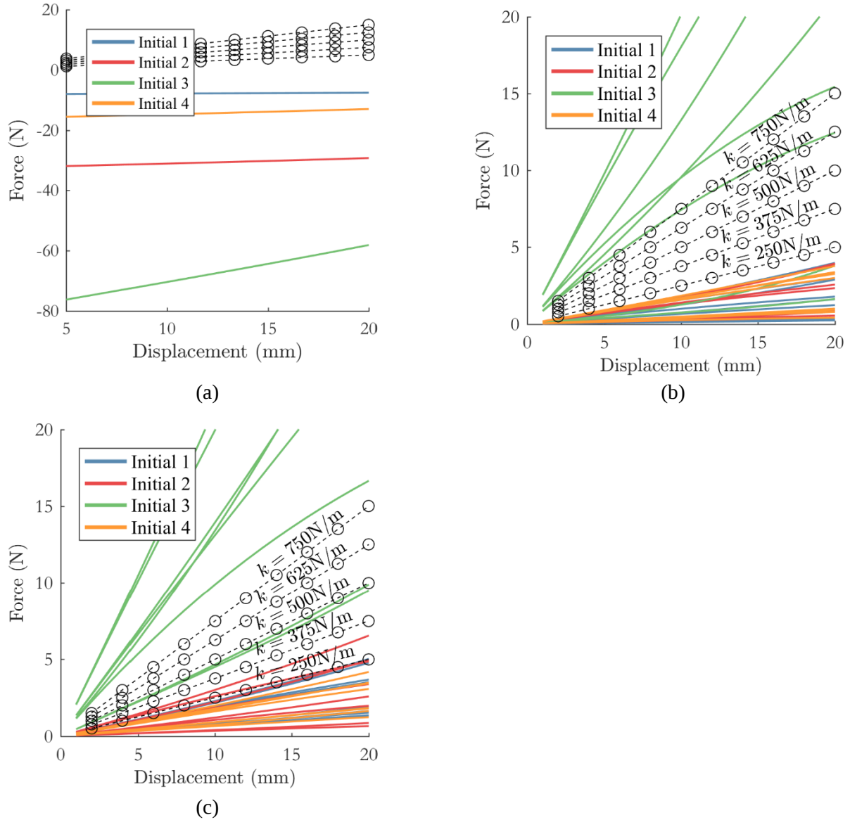
Figure 9 – The axial force profiles of the (un-optimized) initial designs. The same spring designs (indicated by differently colored lines, result in different behaviors for (a) the pinned-pinned spring, (b) the clamped-pinned spring and (c) the clamped-clamped spring. The maximum relative axial error ranges from 70% up to 800%.
