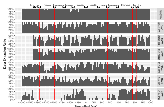
(a) Weak interferer
