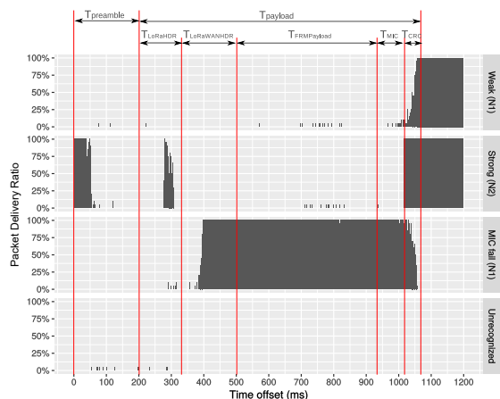
Figure 1: Packet delivery ratio (PDR) for the 2nd scenario.
