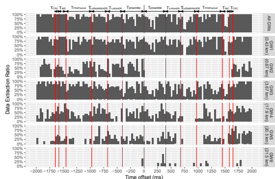
(b) Strong interferer
