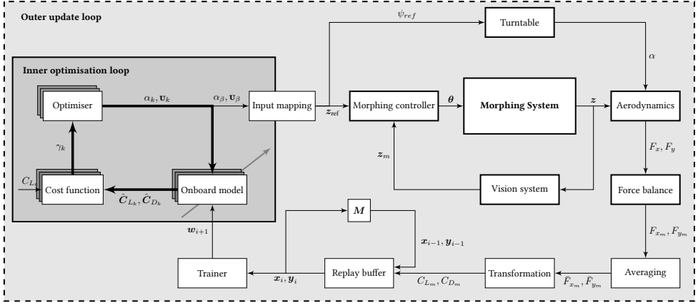
Figure III.3.6: Online shape optimisation architecture diagram with inner optimisation loop and the corresponding components marked in dark gray.
