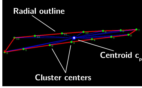
Figure I.1.9: Radial sorting algorithm process. The cluster centres are green dots; the convex radial hull is the red outline.
