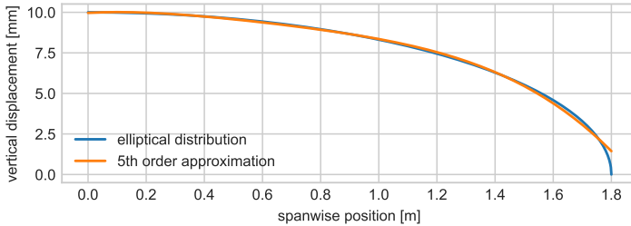
Figure II.2.3: Comparison of an elliptical distribution and 5 th order Chebyshev polynomial approximation.
