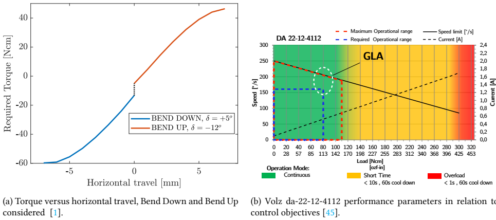
Figure II.1.25: Actuator torque and performance parameters.
