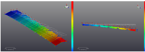
(a) Mode 2 [5.78 Hz]
