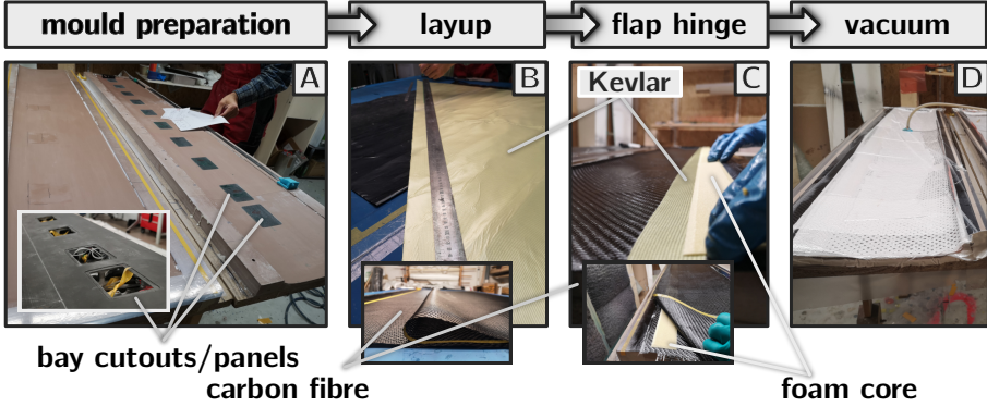
Figure IV.1.8: Manufacturing process.
