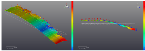
(b) Mode 3 [18.4 Hz]
