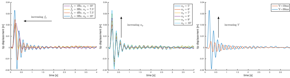
(a) Varying frequency f_g at constant V of 30 ms. (b) Varying gust vane angle \alpha_g at constant V of 30ms and f_g of 5 Hz. (c) Varying free stream velocity V at constant \alpha_g of 10^\circ and f_g 5Hz.
