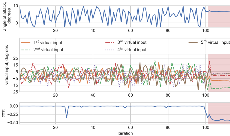
Figure II.2.16: Input history for wandering and optimisation (red background) with C_{L_t} = 0.75 .
