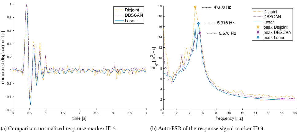
Figure I.1.23: Comparison of the response and the frequency spectrum of the marker ID 3, run R1 (laser versus image tracking).
