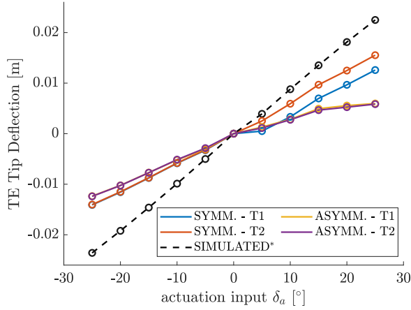
Figure II.1.26: Comparison of tip deflection between the numerical model and DIC measurement of symmetrical and asymmetrical cases [25, -25]^\circ .
