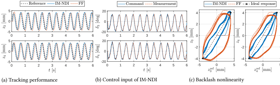
Figure III.2.6: Control performance when tracking a sinusoidal signal with \omega = 12 rad/s, A_m = 4 mm.
