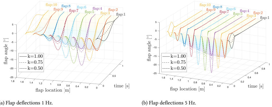
Figure IV.1.15: Spanwise flap deflections comparison for two frequencies and varying scaling parameter.
