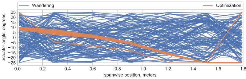
Figure II.2.18: Morphing shapes evaluated on the system in the wandering and optimisation phases.
