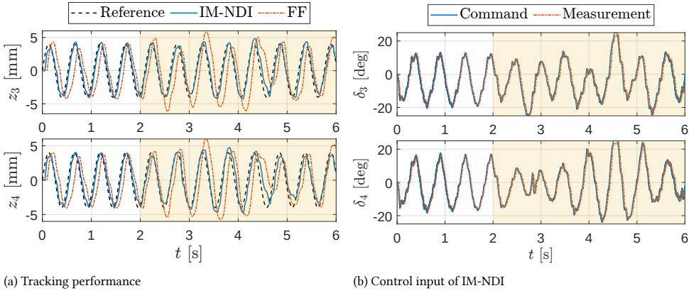
Figure III.2.9: Disturbance rejection performance when tracking a sinusoidal signal with \omega = 12 rad/s, A_m = 4 mm. The shaded area denotes the disturbance injection phase.
