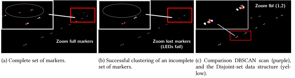
Figure I.1.6: The necessity of unsupervised clustering: incomplete (right, middle) versus full (left) set of markers.
