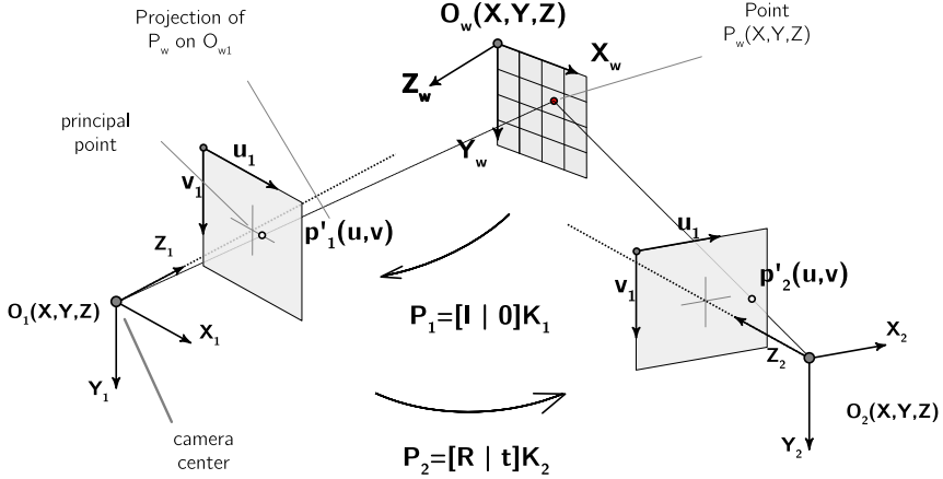
Figure I.2.5: Schematic of the stereo camera setup and the coordinate systems for 3D reconstruction.
