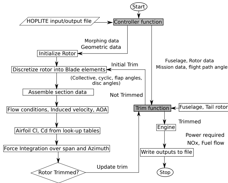
Figure 2: Workflow diagram of rotor module
