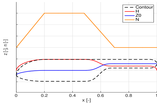
Figure 8: Longitudinal super-ellipse parameter distribution - Side view
