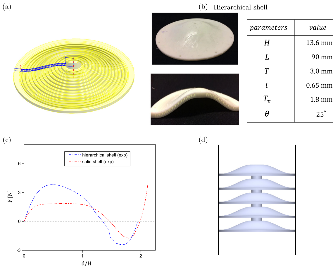
Fig. 10. The lattice-based shell structures. (a) The shell structure is developed by a revolution of the hierarchical beam profile (in blue) along the axis of rotation (red dashed line). (b) A real demonstration of the shell and its cross section. Geometric parameters are depicted. (c) The experimentally characterized force–displacement responses of the hierarchical and the solid shell. (d) An illustration of a serial arrangement of hierarchical shells for energy absorption.
