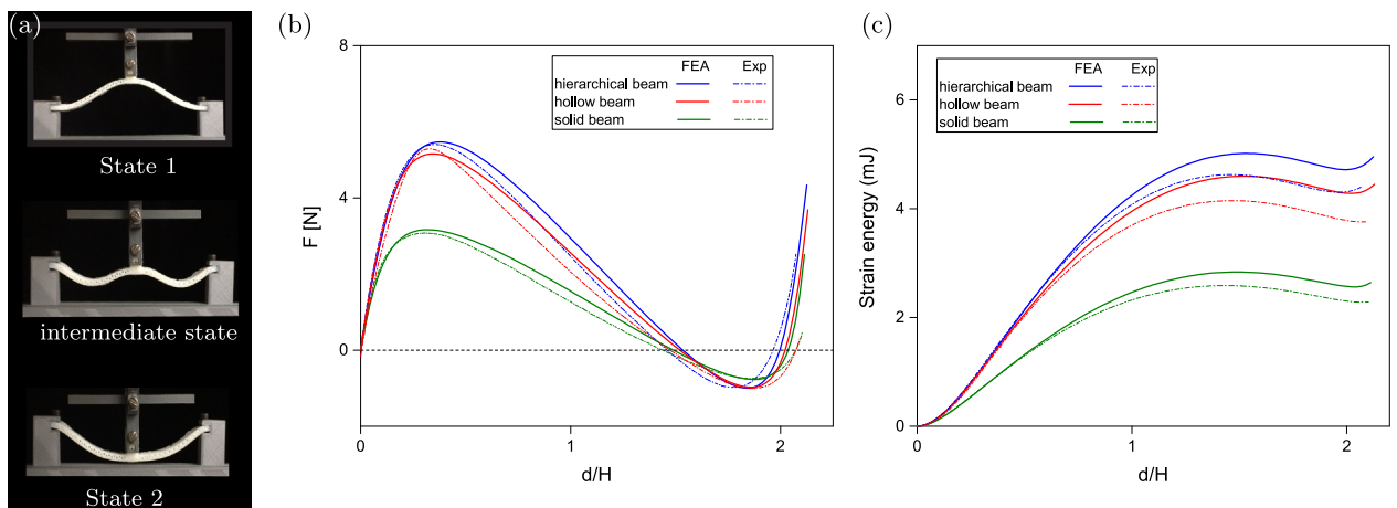
Fig. 3. Snap-through behavior of unit cells. (a) Snapshots of a hierarchical beam during the uniaxial loading. (b) The measured and simulated force–displacement curves of the hierarchical, hollow and solid beams. (c) Evolution of the unit cell's strain energy during the uniaxial loading.
