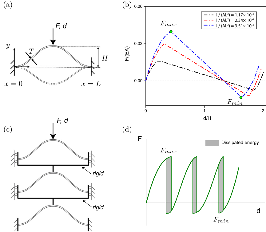
Fig. 1. Pre-shaped solid beams and the effect of bending stiffness on snap-through behavior. (a) A pre-shaped solid beam. The out-of-plane dimension is denoted as B . (b) The force-displacement curves predicted by the analytical model are shown, where cross-sectional area is kept as a constant value ( A = 12 \text{ mm}^2 ). Snap-through responses of beams with different relative bending stiffness are presented. (c) A system composed of three pre-shaped beams arranged in series. (d) The force-displacement curve of the three-beam system under a displacement-controlled loading cycle is illustrated.
