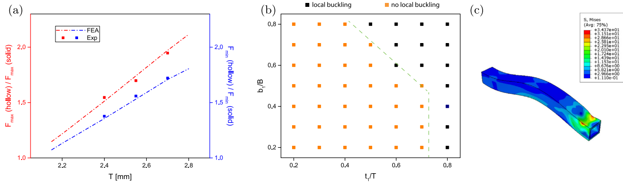
Fig. 5. Tuning the critical loads for the hollow beam. (a) Experimentally and numerically characterized critical loads are plotted as a function of T . (b) The effect of the inner cross-sectional parameters ( b_1 and t_1 ) on local buckling. (c) The local buckling of the hollow beam.
