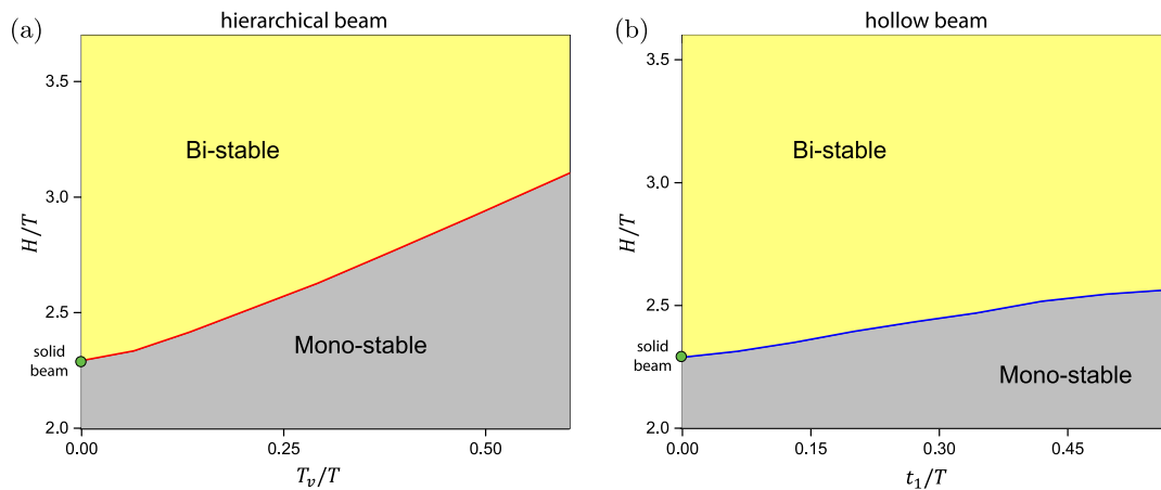
Fig. 6. The bi-stable criterion for the hierarchical and hollow beam. (a) With changing H/T and T_v/T , the bi-stable region for hierarchical beams can be identified. (b) For the hollow beam, the bi-stable region is plotted as a function of H/T and t_1/T .
