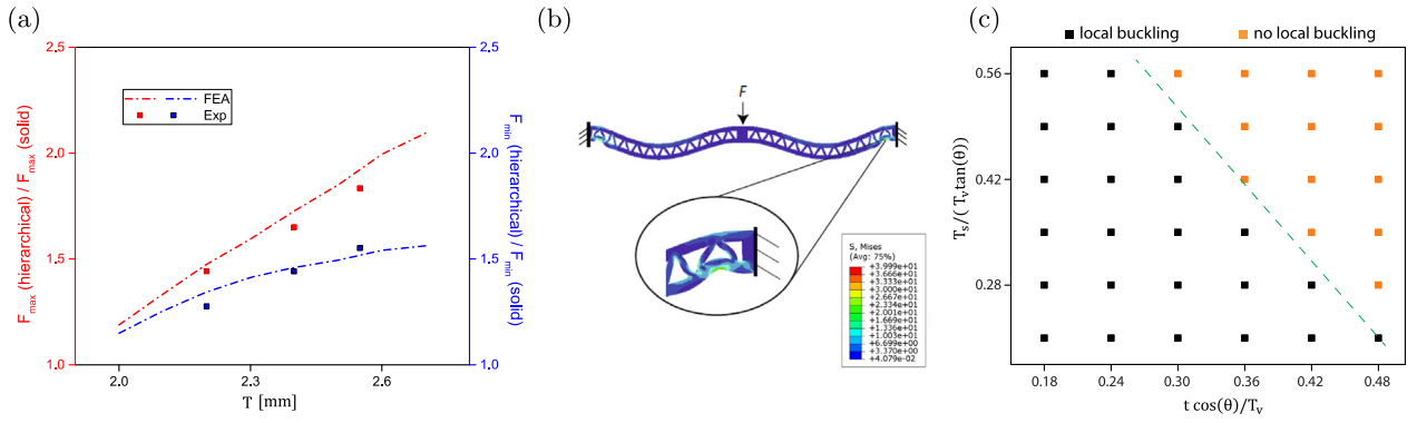
Fig. 4. Tuning the hierarchical beam's snap-through behavior via varying the thickness T . (a) Experimentally and numerically characterized critical loads as a function of T . (b) The local buckling. (c) Effect of the lattice parameters on the local buckling.
