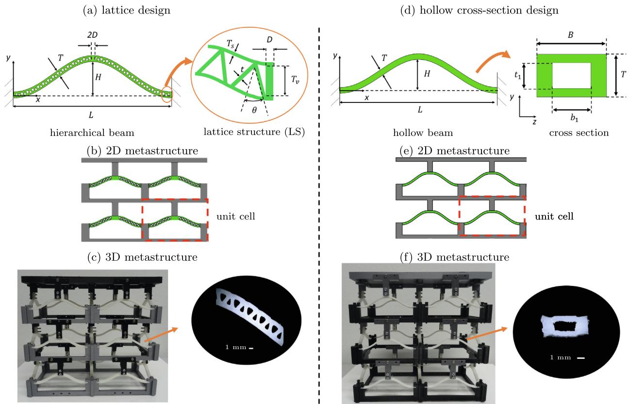
Fig. 2. A schematic of the proposed designs. (a)–(c): The developed lattice-based metastructures. Geometric parameters of the hierarchical beam are depicted in (a). (d)–(f): Metastructures based on hollow beams with box-shaped cross sections.
