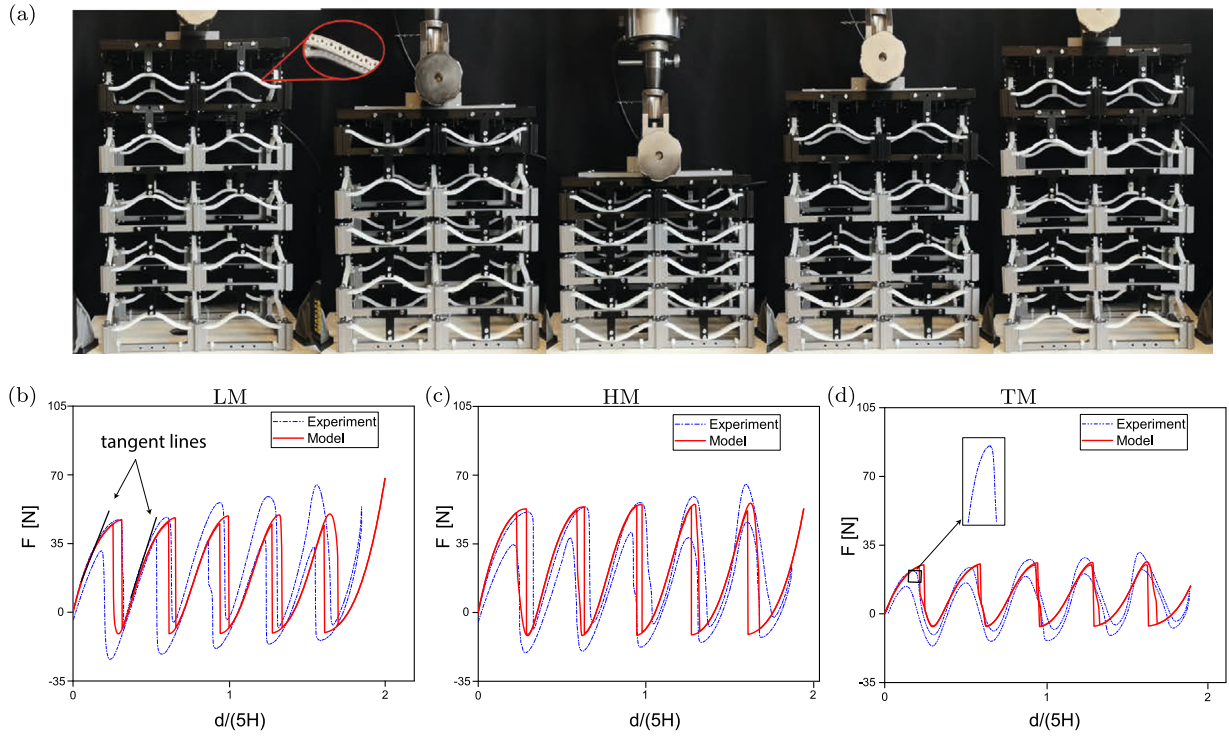
Fig. 7. Mechanical responses of multi-stable metastructures under displacement-controlled cyclic loading. (a) Different deformation stages of the LM in a loading–unloading test. (b)–(d) Force–displacement curves of the LM, HM, and TM under a complete displacement-controlled loading and unloading cycle.
