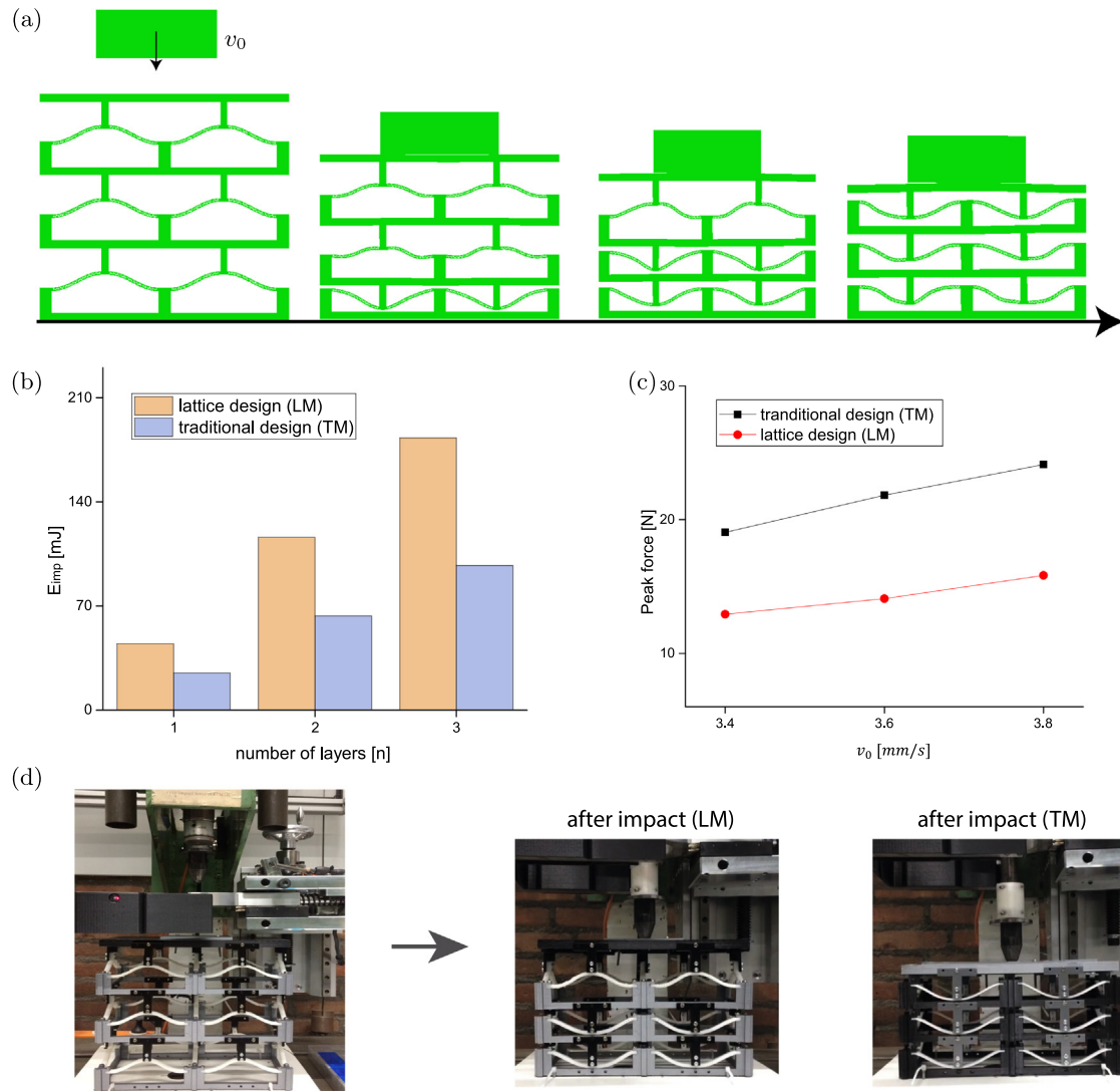
Fig. 9. Protective capability of multi-stable metastructures. (a) Different stages of metastructures' deformations under an impact. (b) The simulated critical mechanical energy ( E_{imp} ) of the LM and TM. (c) Simulated peak forces for the TM and LM design. (d) Experimental demonstration of the impact performance for the LM and TM.
