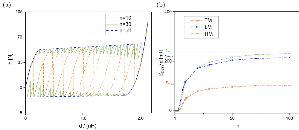
Fig. 8. Energy dissipation of n -layer metastructures. (a) The predicted force–displacement curves of n -layer metastructures. (b) The comparison between the LM, HM, and TM in terms of energy dissipation. E_{max} represents the maximal energy that can be dissipated per layer in a load-unloading process.
