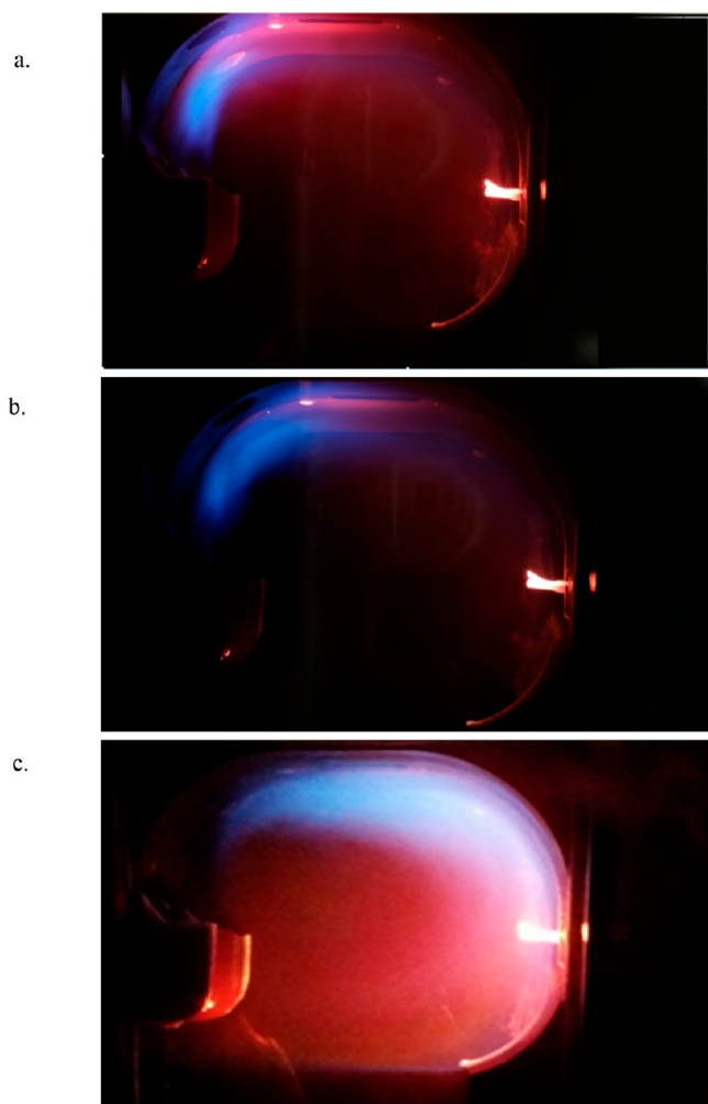
Figure 4. Photographs of the combustor for different amounts of N_2 addition. 30 For 0 l_n/min , 40 l_n/min and 100 l_n/min steps (from a to c). Fuel mass flow of 5.91 \times 10^{-5} kg/s. The incandescent filament on the right side is a thermocouple. Please note that the photographs are meant for visual representation only.
