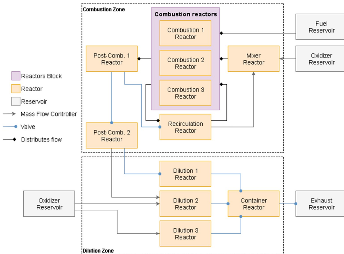
Figure 14. Structure of the designed CRN.
