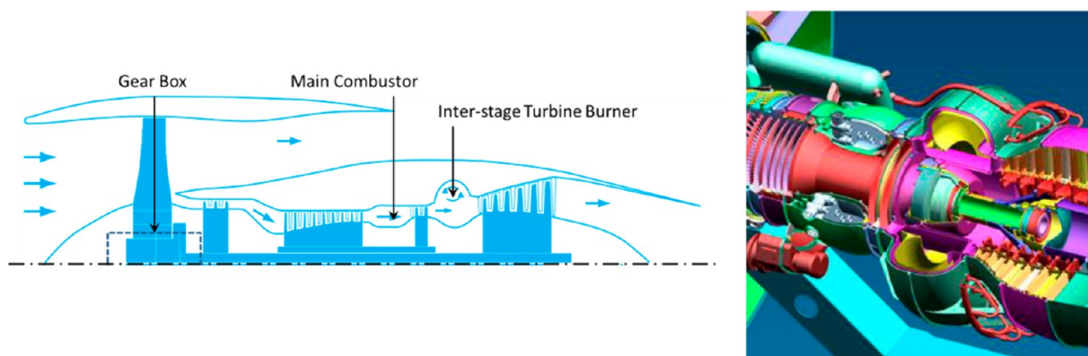
Figure 2. Dual-combustor engine concept presented along with the AHEAD project (left). 19 Cut-view of the ITB on the full engine structure. Right panel: Copyright 2014 Pratt and Whitney Rzeszów S.A.
