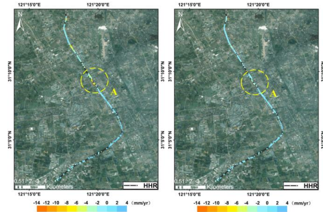
(a) Vertical deformation rate (b) West-east deformation rate Fig. 12. Vertical and west-east deformation rate maps of HHR combining ASAR and TSX images (2008-2010). Background image: Google Map.
