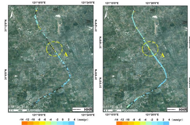
(a) LOS deformation rate from ASAR (b) LOS deformation rate from TSX Fig. 11. LOS deformation rate map of HHR (2008-2010). Background image: Google Map.
