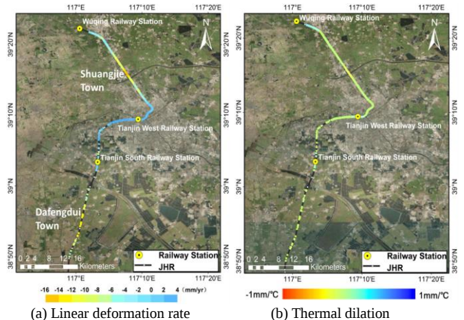
Fig. 5. Linear deformation rate and thermal dilation maps of JHR (2008-2009). Background image: Google Map.
