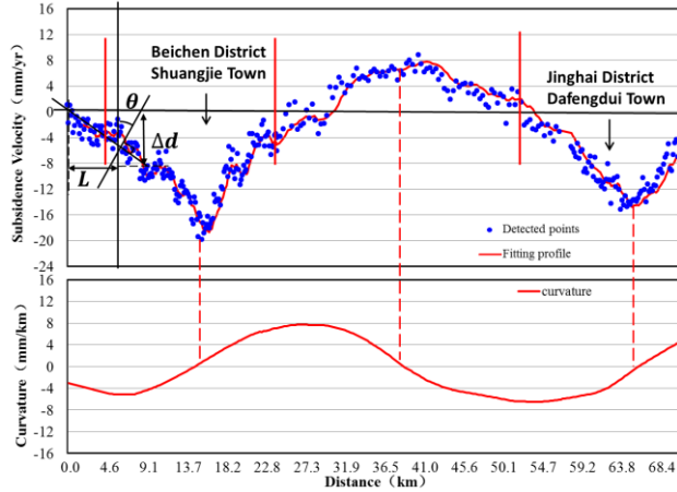
(b) Subsidence rate profile and curvature of JJR Fig. 8. Vertical subsidence rate, profile and curvature of JHR (2008-2009)
