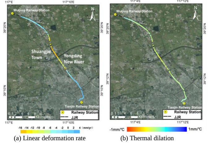
Fig. 4. Linear deformation rate and thermal dilation maps of JJR (2008-2009). Background image: Google Map.
