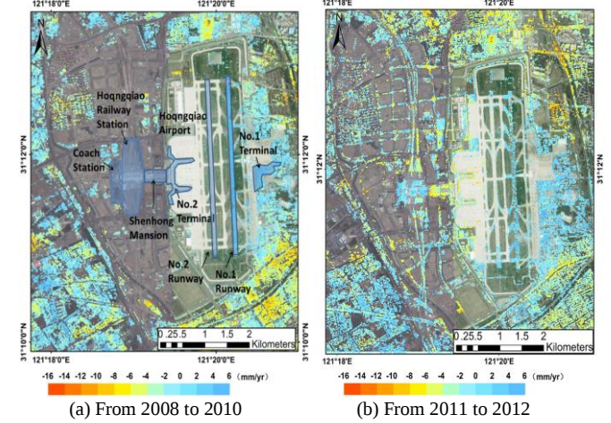
(a) From 2008 to 2010 (b) From 2011 to 2012 Fig. 14. Deformation rates of Hongqiao Hub during two different periods. Background image: Google Map.
