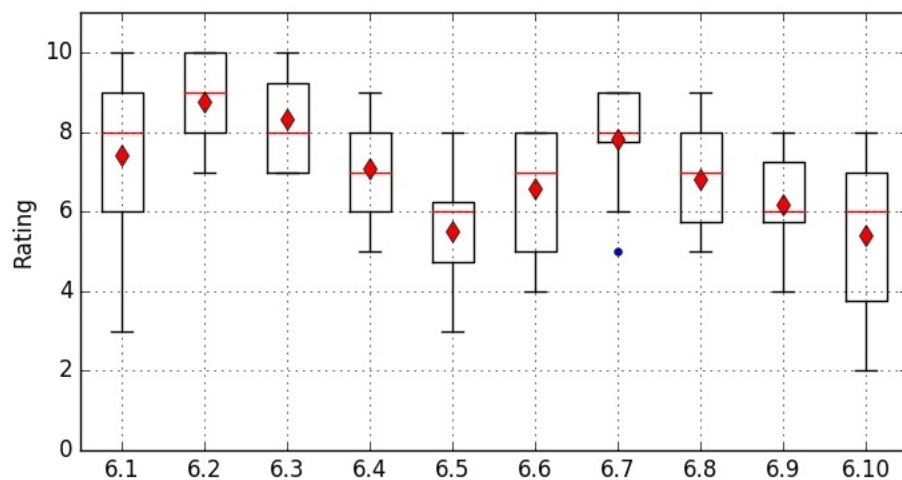
Fig. 8 Box plot survey results o question group 6 [n=12].
