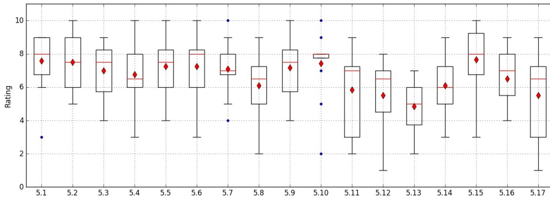
Fig. 7 Box plot survey results question group 5 [n=12].
