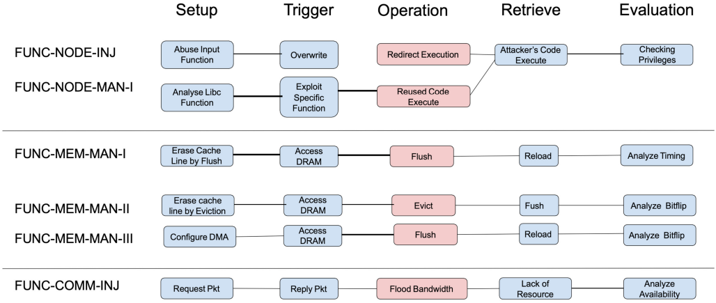
Fig. 6. Attack phases of functionality attacks and groups.
