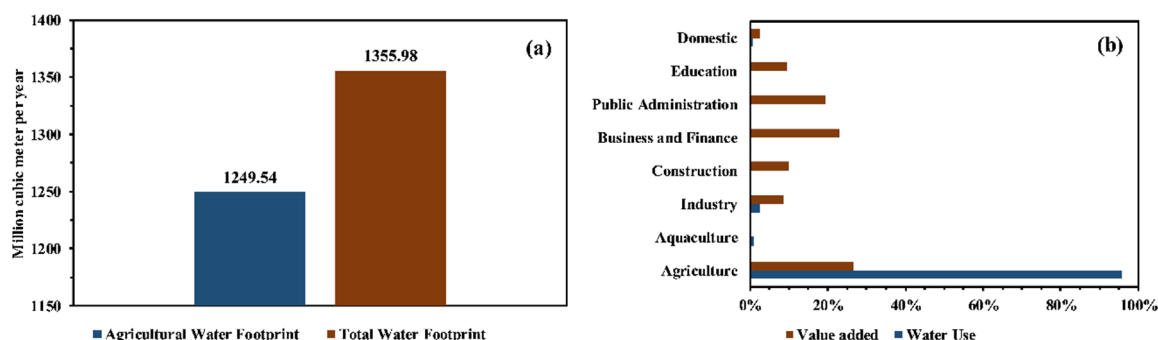
Figure 2. (a) Comparison between agricultural water footprint and total water footprint, and (b) the contribution of each economic sector in water use and value-added.
