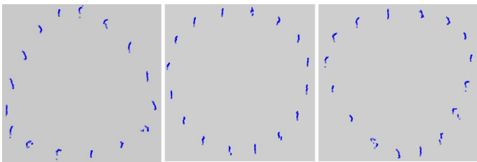
Figure 4.21: Resulting operational mode shape at 86Hz.
