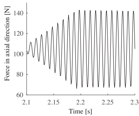
Figure 5.18: a) The applied load in axial direction of 100 Hz that is applied after 2.1 s and gradually increased in amplitude.
