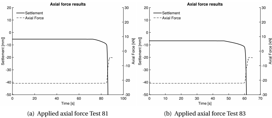
Figure B.26: The applied axial loads during the dismounting tests with slip-joint set 1 of the eight batch of the experiments.
