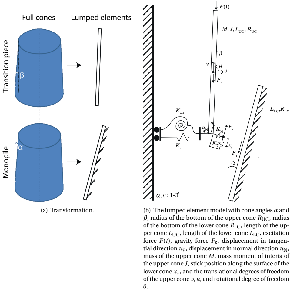
Figure 3.1: (a) Transformation from full cones to lumped elements and (b) the adopted lumped model.
