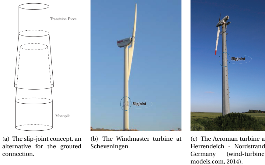
Figure 1.3: The slip-joint concept and two existing onshore turbines with a slip-joint connection.
