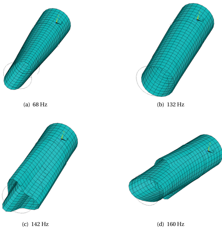
Figure 5.5: Modes shapes 1-4 of the combined system after initial settlement.
