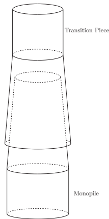
Figure 2.1: The slip-joint.
