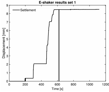
(a) Test 58; F_{ax}=10 kN
