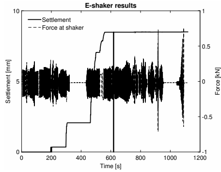
(b) Force at shaker Test 58
