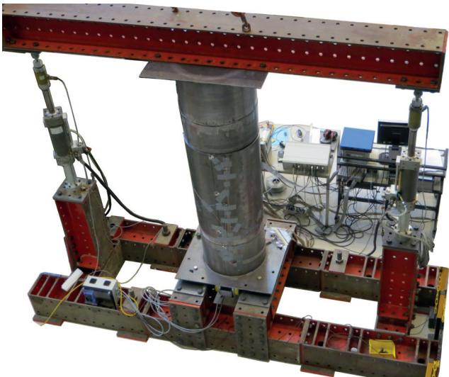
Figure 4.2: The experimental setup as built in the Stevinlab in Delft.
