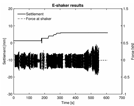
(f) Force at shaker Test 63
