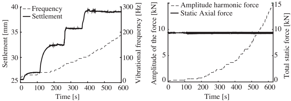
(a) The settlement of the upper cone and the vibrational frequency, Test 1.
