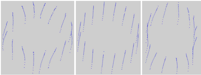
Figure 4.23: Resulting operational mode shape at 120Hz.
