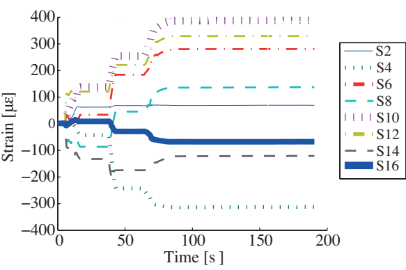
Figure 4.13: Strain gauges results at 10cm from the open end.
