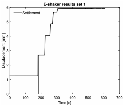
(e) Test 63; F_{ax}=10 kN
