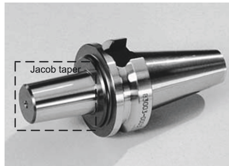
(b) Jacob taper holder (Nikken, 2015)
