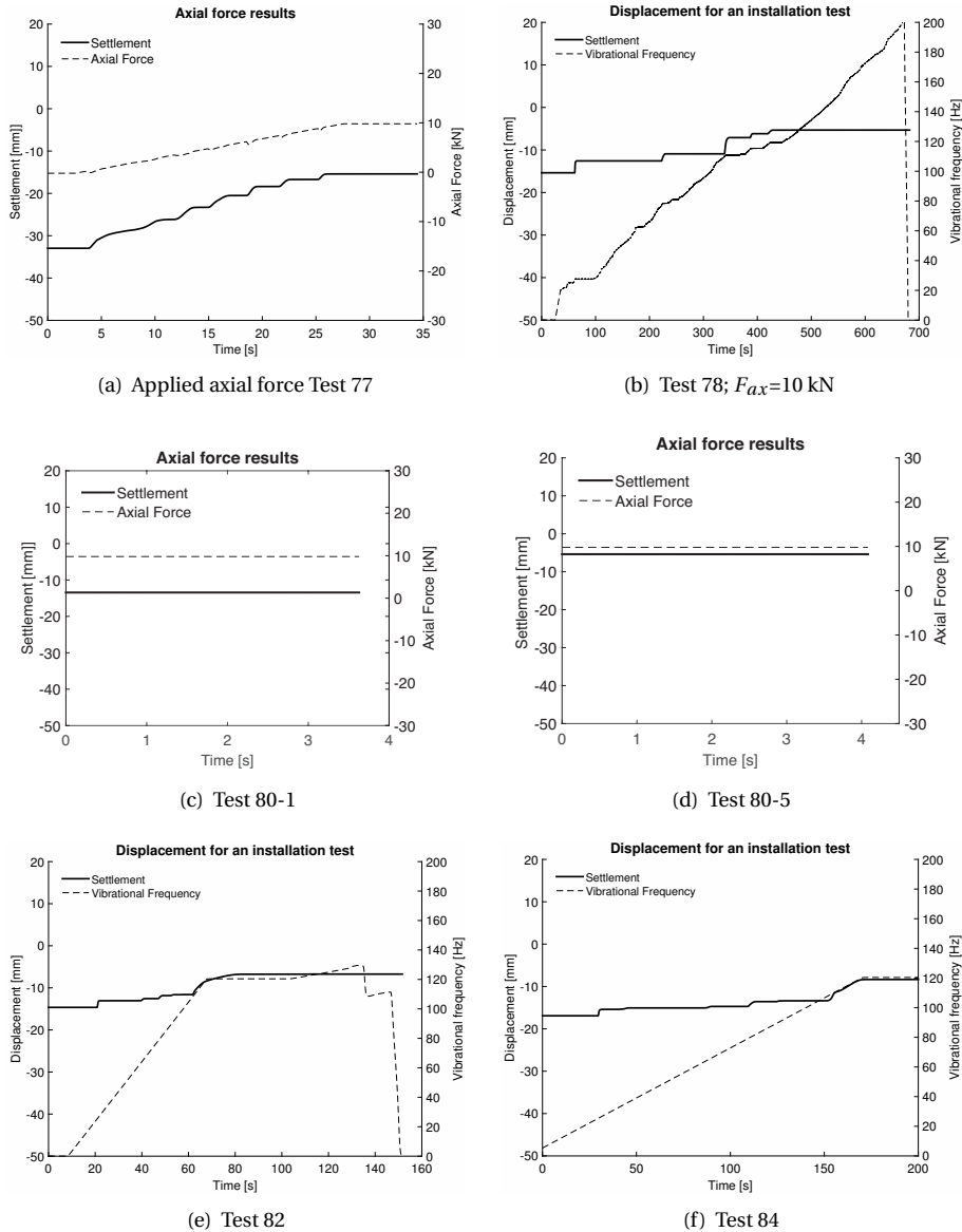
Figure B.24: The measured settlement of the upper cone, the applied axial load and the frequency of the applied vibration in the installation tests with slip-joint set 1 of the eight batch of experiments
