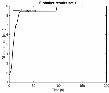
(c) Test 60; F_{ax}=10 kN - 119 Hz
