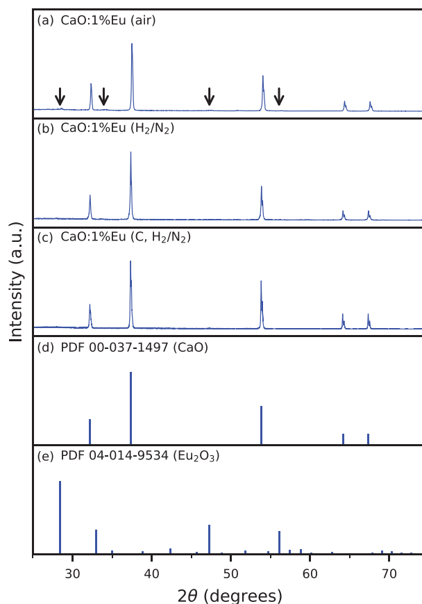
Figure 1. X-ray diffractograms of a) \text{CaO}:\text{1at.}\%\text{Eu} (air), b) \text{CaO}:\text{1at.}\%\text{Eu} ( \text{H}_2/\text{N}_2 ), and c) \text{CaO}:\text{1at.}\%\text{Eu} (C, \text{H}_2/\text{N}_2 ). ICDD reference patterns d) \text{CaO} (PDF 00-037-1497), and e) \text{Eu}_2\text{O}_3 (PDF 04-014-9534).
