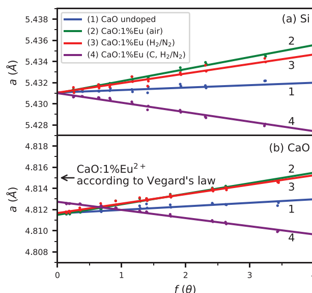
Figure 2. Lattice parameter a as a function of f(\theta) for a) Si internal standard and b) \text{CaO} samples. The real lattice parameter is found at f(\theta) = 0 .
