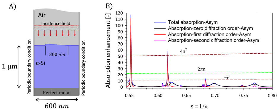
Fig. 8. (A) shows one period of a 1- \mu\text{m} thick Si slab endowed with an asymmetric grating. The grating has a period of 600 nm, duty cycle 50% and height of 20 nm. The structure is excited using normal incidence plane wave. The electric field inside the Si slab is calculated using COMSOL multiphysics. (B) Shows the absorption enhancement in the structure shown in (A), total absorption at each wavelength is divided by the one pass absorption [43] at corresponding wavelength, to calculate the enhancement. Absorption enhancement for each grating order is also presented in different color.
