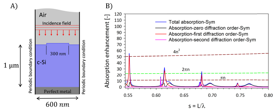
Fig. 7. (A) shows one period of a 1 \mu\text{m} thick Si slab endowed with a symmetric grating. The grating has a period of 600 nm, duty cycle 50% and height of 20 nm. The structure is excited using normal incidence plane wave. The electric field inside the Si slab is calculated using COMSOL multiphysics. (B) Shows the absorption enhancement in the structure shown in (A), total absorption at each wavelength is divided by the one pass absorption [43] at corresponding wavelength, to calculate the enhancement. Absorption enhancement for each grating order is also presented in different color.
