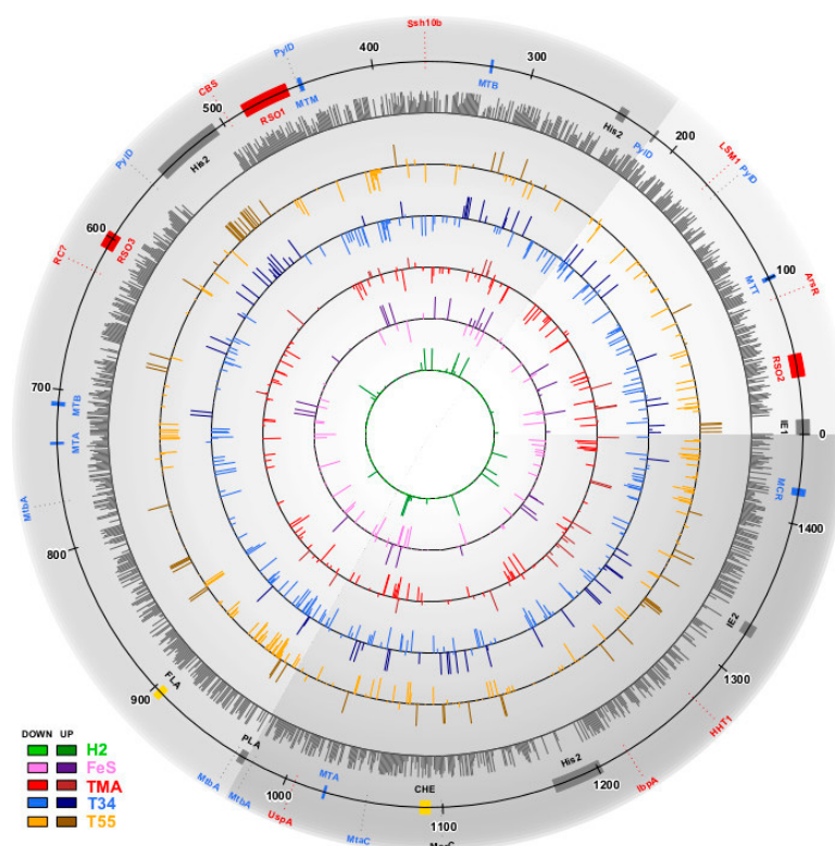
Figure 1. Schematic map of protein expression in different conditions along the Methanonastronarchaeum thermophilum AMET1 genomic contigs. The grey transparent sectors show M. thermophilum AMET1 genomic contigs as follows: AMET1_2—light grey, AMET1_3—medium grey, AMET1_4—dark grey (minor contigs are not shown). Dark grey circle shows base (optimal) conditions relative protein abundance level. The inner cycles represent up- and down regulated genes in different experimental conditions according to the colour code shown on the left bottom corner of the Figure. Genes and genes clusters described in the paper shown by shapes and lines as follows: Red—the most abundant genes; Red—RSO1,2,3—three ribosomal; Blue—methanogenesis related genes; Blue—methanogenesis operons: MTT—trimethylamine-corrinoid methyltransferase, MTB—dimethylamine-corrinoid methyltransferase superoperons; MTM—methylamine-corrinoid methyltransferase, MTA—methanol-corrinoid methyltransferase; MCR—methyl coenzyme M reductase; Yellow—chemotaxis operon (CHE) and archaellum (FLA). Black—mobile elements: His2—His2 virus related loci, PLA—putative plasmid, IE1 and IE2—integrated elements.
