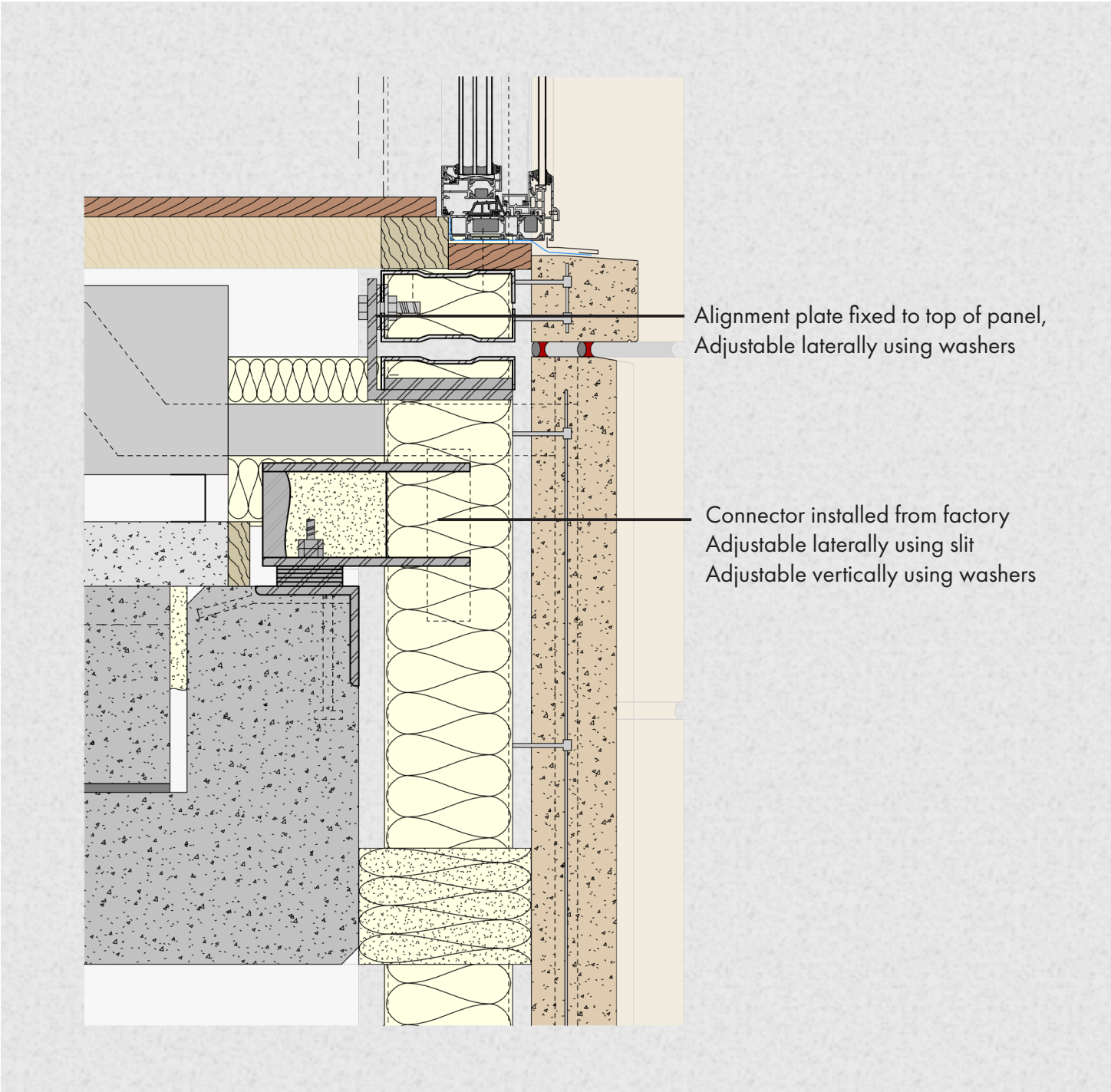
Load Bearing Panel Connection
