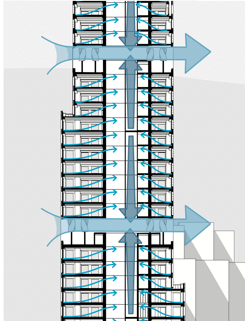
Zoom: Ventilation
