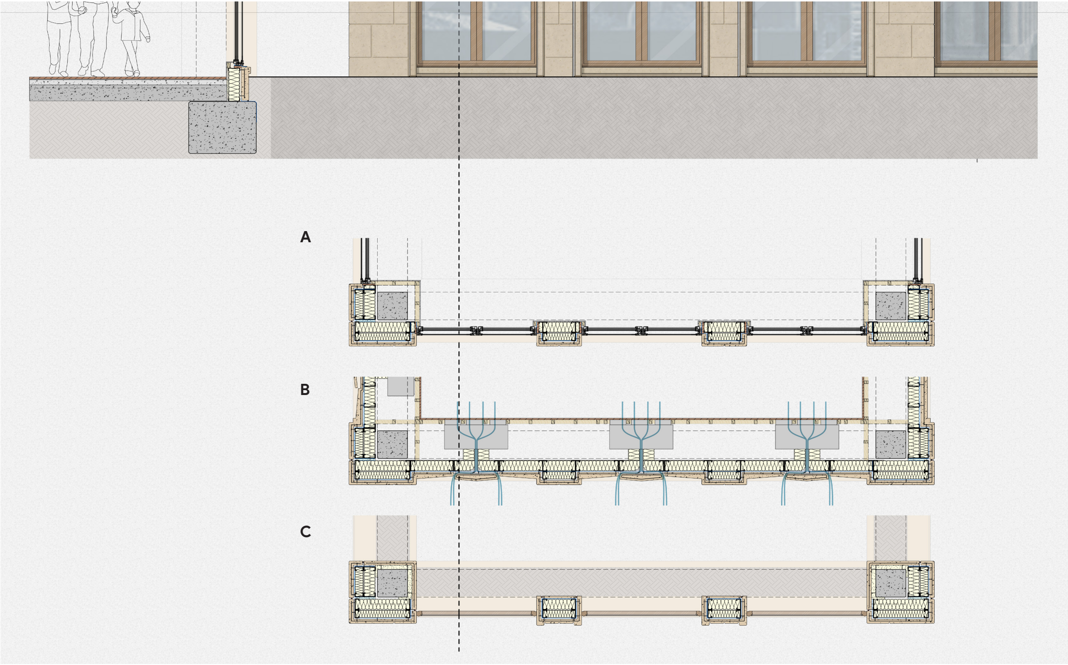
Zoom 3: Ground Floor Connection - Horizontal Sections
