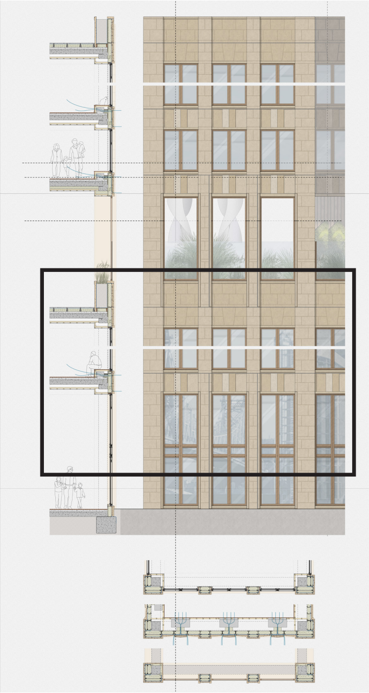
Overview Complete Fragment
