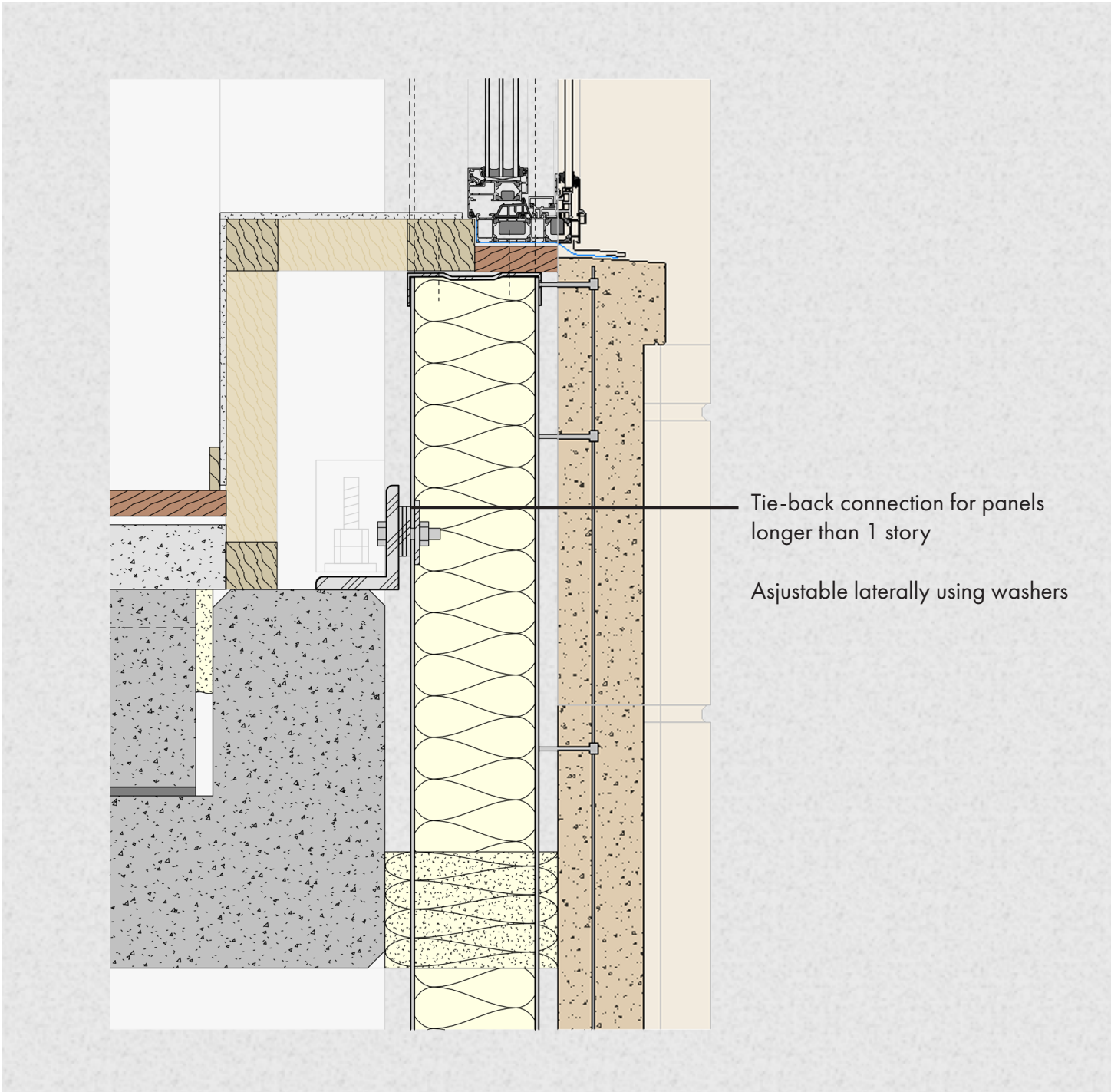
Tie - Back Panel Connection
