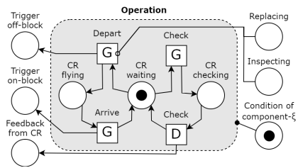
Fig. 10. SDCPN model of the flight crews.
