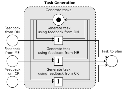
Fig. 6. SDCPN model of the task generating team.
