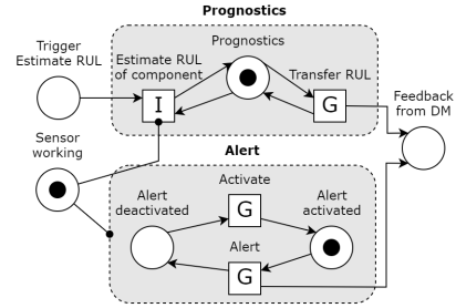
Fig. 9. SDCPN model of the data management team.
