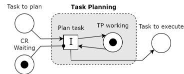
Fig. 7. SDCPN model of the task planning team.
