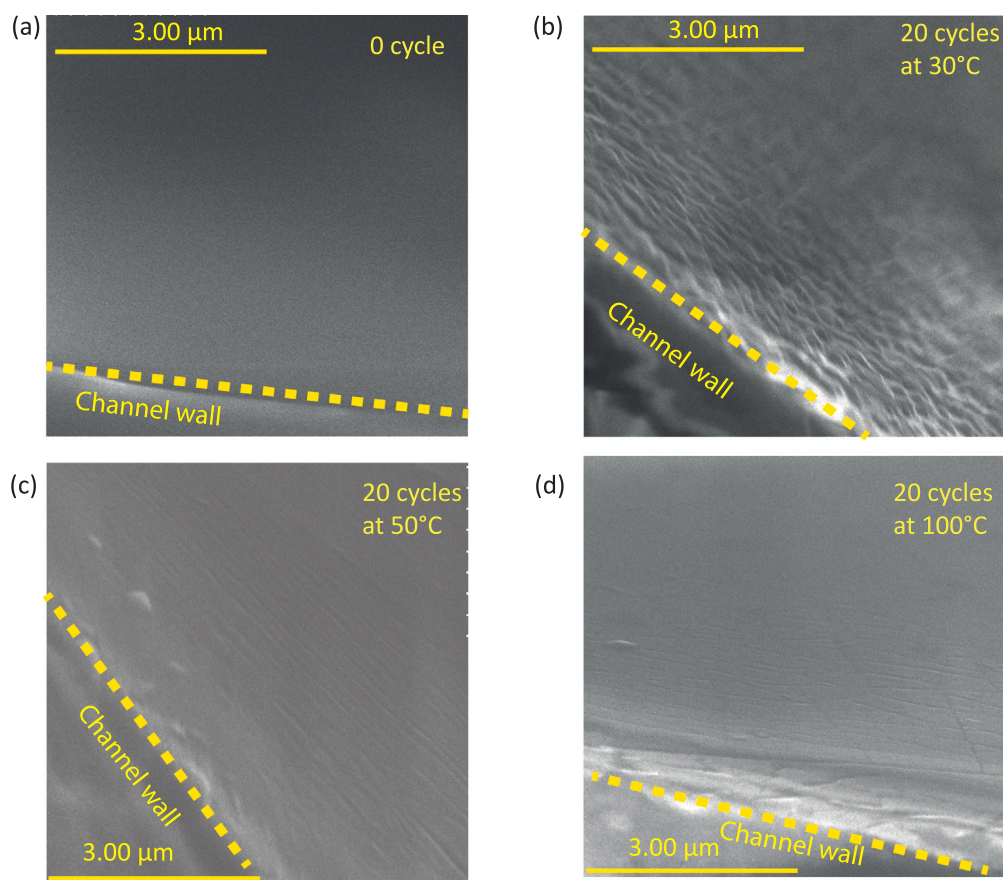
Fig. S3. FE-SEM images of bare and \text{SiO}_x -coated PDMS chips obtained after making cross-sectional cuts of the chips that feature a straight 11.6 mm long, 500 μm wide, and 50 μm high microchannel. \text{SiO}_x AP-ALD treatment: 20 ALD cycles at 30 °C, 50 °C, and 100 °C.
