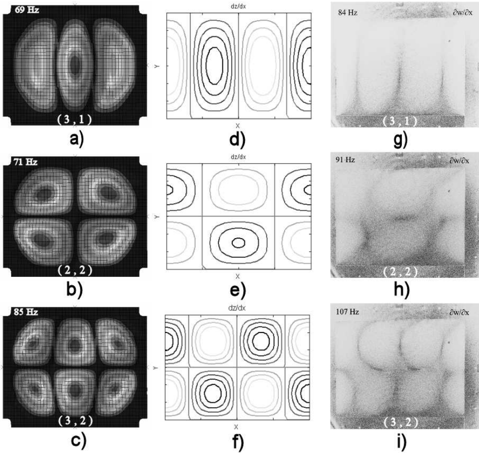
Figure 5.8: Mode shapes (3,1), (2,2), (3,2), predicted by FE model (left, a, b, c) and measured mode shapes with laser shearography (right, g, h, i) for Amazoné linen with cracked ground 40 x 30 cm. Shearography mode shape measurements g)(3,1), h)(2,2) and i)(3,2) show displacement derivatives with respect to the x direction. The analytical mode shape derivatives (middle d, e, f) are given to allow for a direct comparison between the predicted mode shapes (a, b, c) and the measured mode displacement derivatives (g, h, i).
