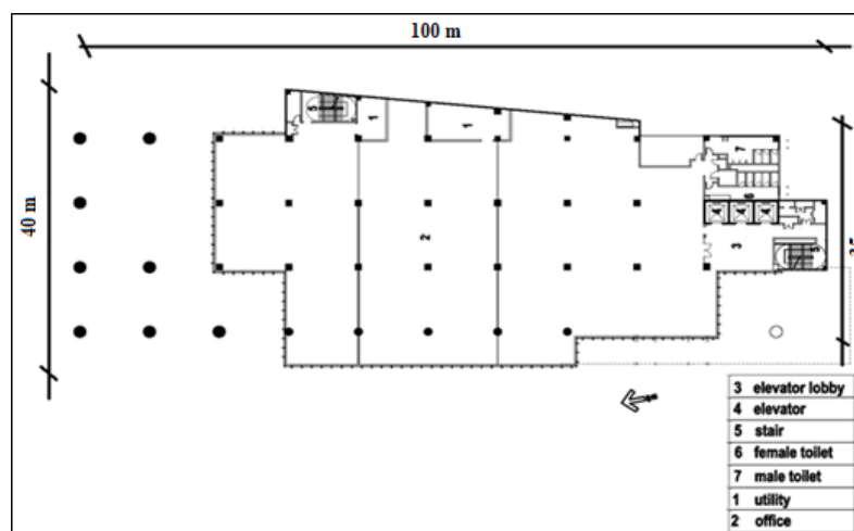
Figure 3. Plan layout of the selected office building—open plan office.
