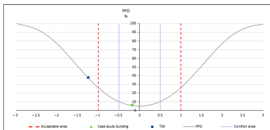
Figure 10. TSV versus Fanger's PMV-PPD model.
