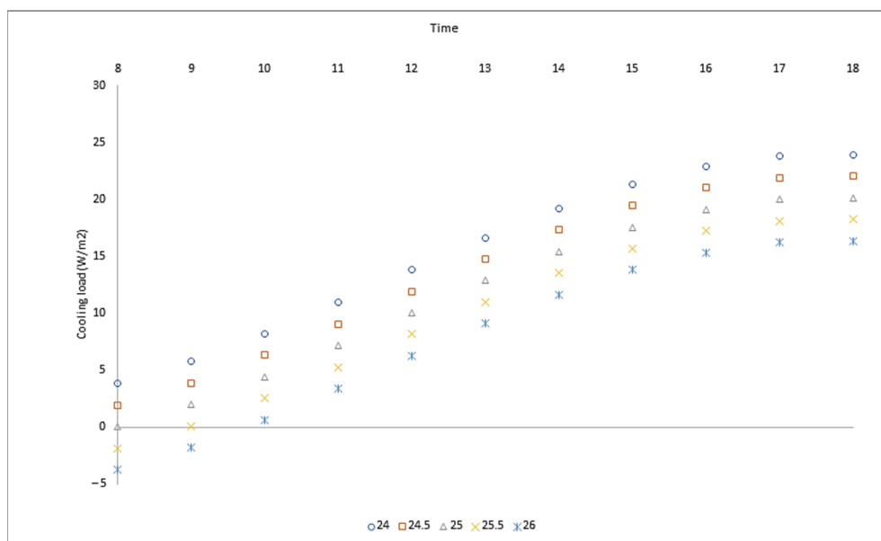
Figure 15. Hourly cooling load in different temperatures.
