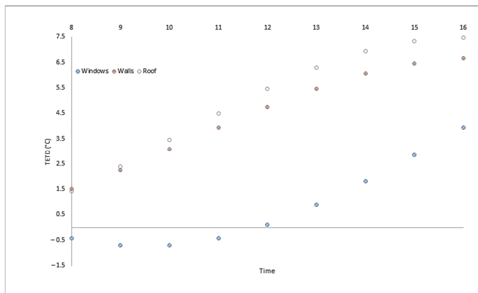
Figure 14. TETD of building envelopes at 24 °C.
