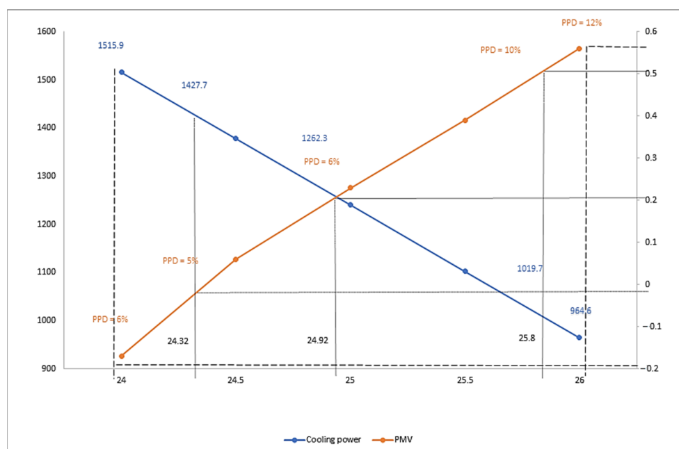
Figure 17. Optimum temperature based on PMV and cooling power.
