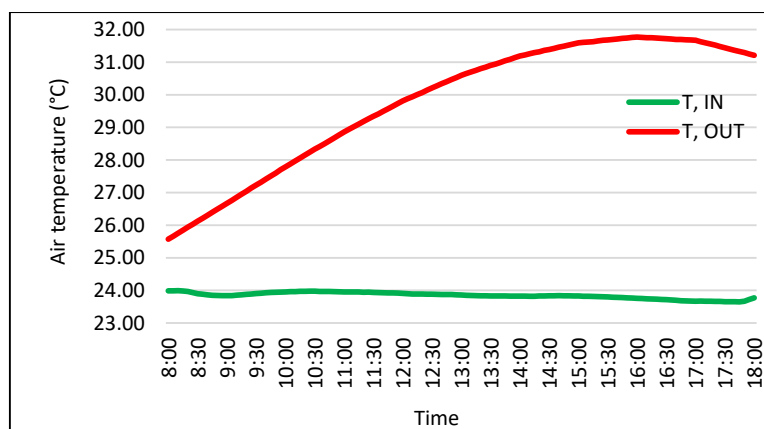
Figure 11. Indoor vs. outdoor temperature.
