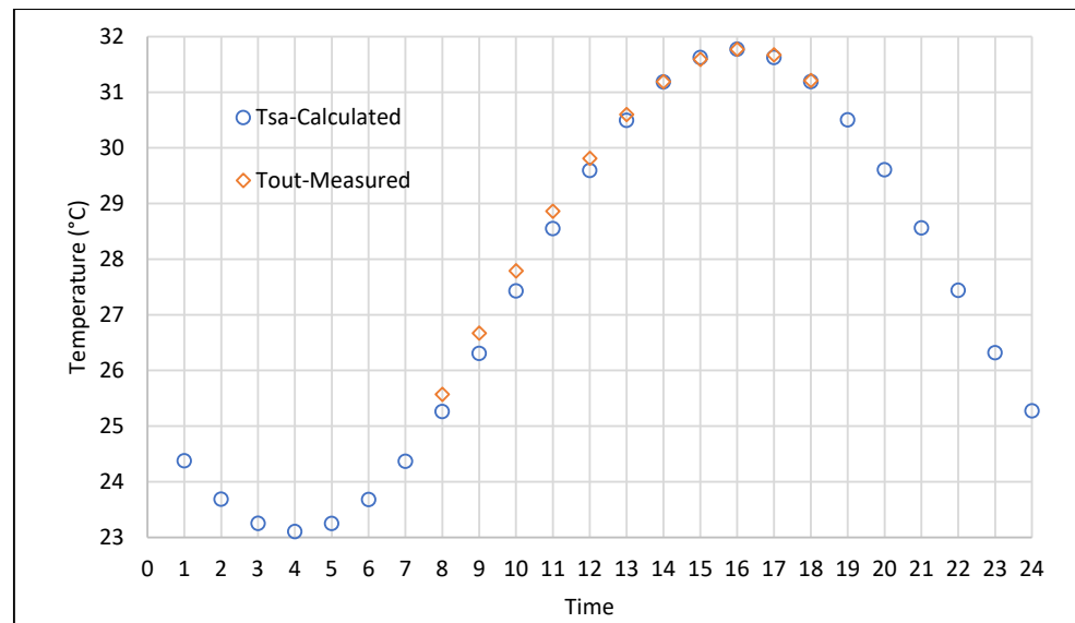
Figure 13. Sol-air and outdoor temperature.
