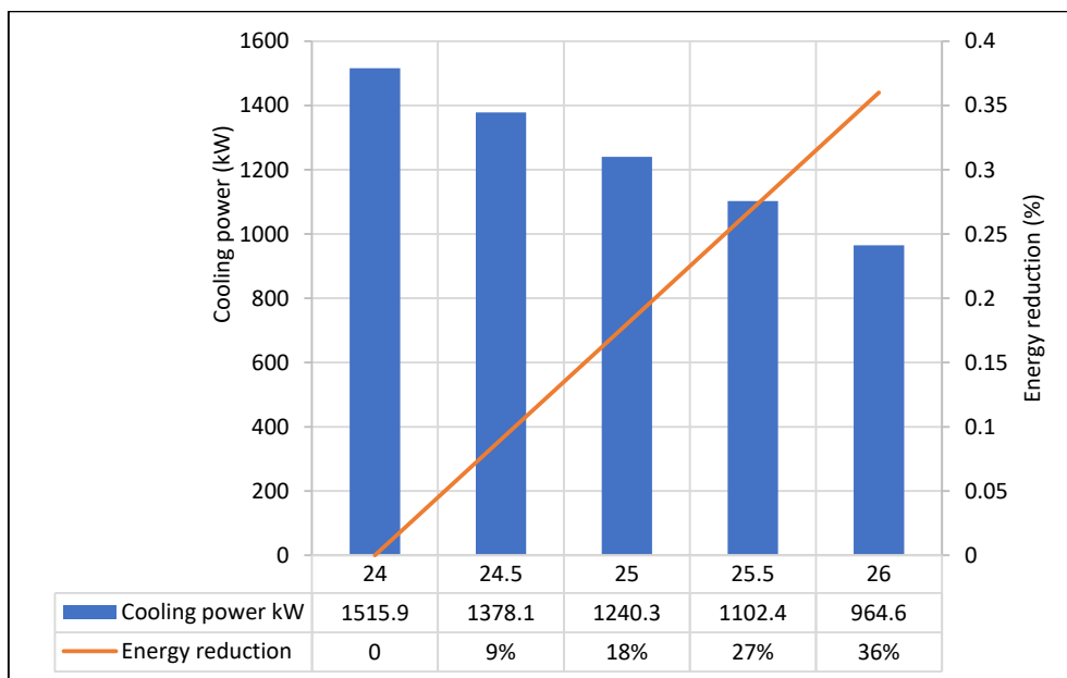
Figure 16. Total cooling load in different temperatures.
