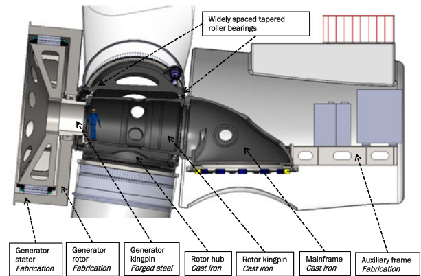
Fig. 1. Cross section view of the INNWIND.EU nacelle with the 10 MW \text{MgB}_2 generator mounted in front of the turbine blades [12]. The inner and stationary structure of the generator is attached to the stationary kingpin going through the rotor hub and connected to the main frame.
