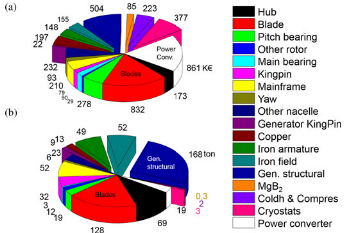
Fig. 3. 10 MW \text{MgB}_2 superconducting direct drive wind turbine rotor, generator and nacelles component cost and weight breakdown [11]. a) Component cost in [k€] and b) component weight in [ton] according to the components outlined in [12]. The components associated with the superconducting drive train have been displaced from the center.
