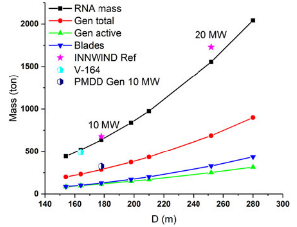
Fig. 2. Mass scaling of the main components of the front mounted \text{MgB}_2 superconducting direct drive generator as function of the turbine rotor diameter [11]. The \text{MgB}_2 generator active materials mass (green) are added to the structural generator mass whereby the total generator mass (red) is obtained. By adding also the blade mass (blue) and the nacelle mass then the Rotor Nacelle Assembly (RNA) mass (black) is obtained. The RNA of the INNWIND.EU reference designs for P = 10 MW and 20 MW are shown (stars) as well as the RNA of the Vestas V-164 [17] and the total generator mass of a 10 MW permanent direct drive generator design by Polinder [9].
