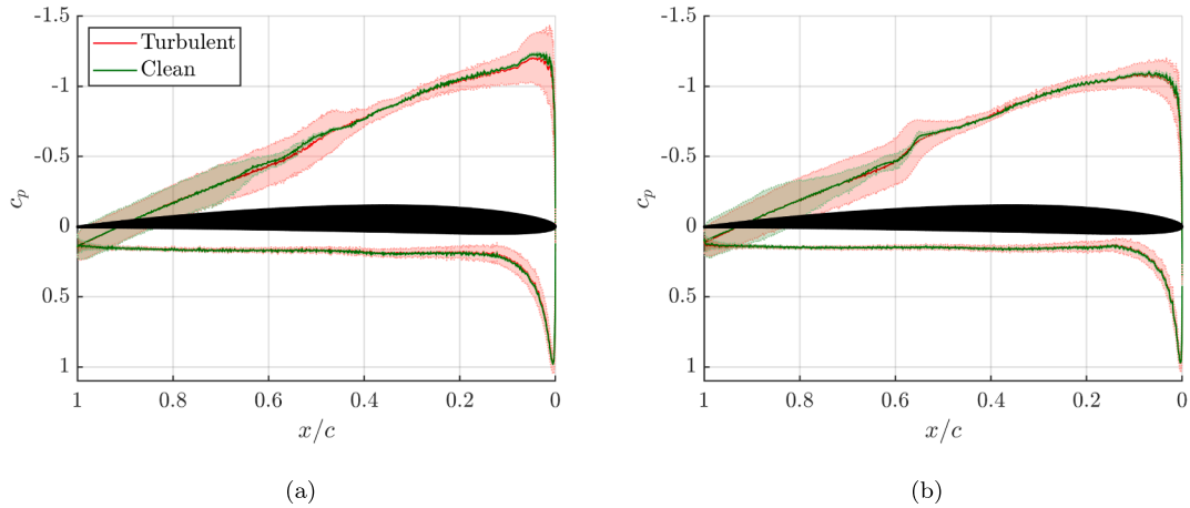
Fig. 20. c_p at r/R = 0.6 (a) and 0.7 (b) under turbulent (—) and clean (—) inflow conditions. The width of the shaded region identifies the c_{p,rms} .
