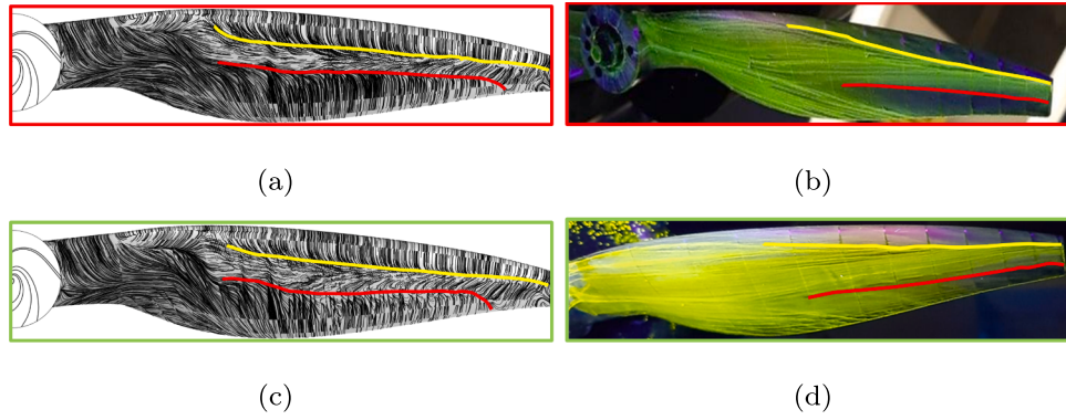
Fig. 5. Time-averaged surface streamlines and oil flow under (a-b) turbulent and (c-d) clean inflow. Yellow and red lines indicate separation and transition, respectively. For interpretation of the references to colour in this figure legend, the reader is referred to the web version of this article.
