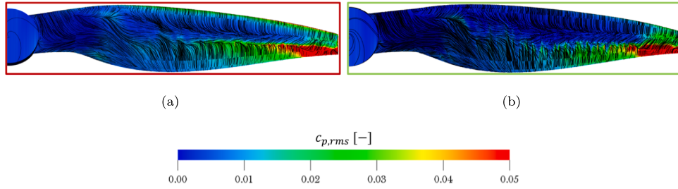
Fig. 19. c_{p,rms} and time-averaged surface streamlines under (a) turbulent and (b) clean inflow conditions.
