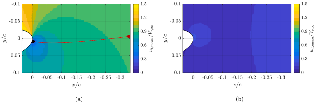
Fig. 14. u_{t,\text{mean}} and w_{t,\text{mean}} close to the leading edge at r/R = 0.6 . The red line in Fig. 14a individuates the local stagnation line. The spectrum of the upwash velocity v_t shown in Fig. 16 is computed at the red and black points. For interpretation of the references to colour in this figure legend, the reader is referred to the web version of this article.
