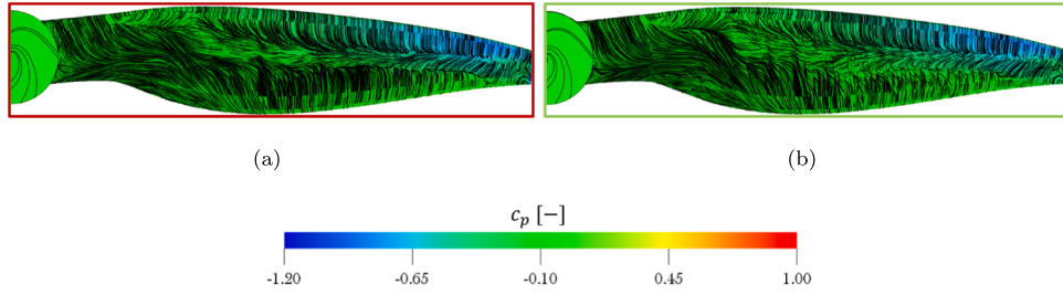
Fig. 18. Time-averaged c_p and surface streamlines under (a) turbulent and (b) clean inflow conditions.
