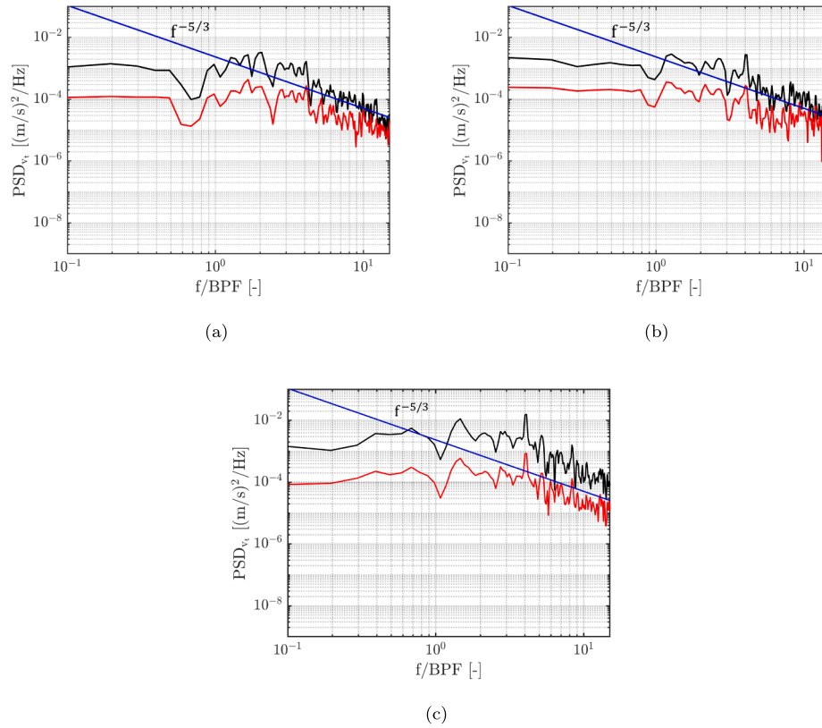
Fig. 16. PSD of the upwash velocity v_t computed (a) at the red and black points shown in Fig. 14 at r/R = 0.6 and at corresponding points along the stagnation line at (b) r/R = 0.7 and (c) r/R = 0.9 . Line colors refer to the sampling points in Fig. 14. For interpretation of the references to colour in this figure legend, the reader is referred to the web version of this article.
