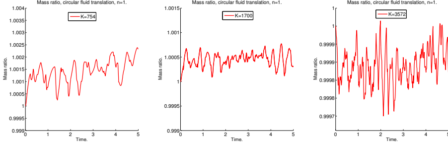
Figure 2.4: Evolution of M(t)/M(0) for the translation of a LS representation of a circular interface.
