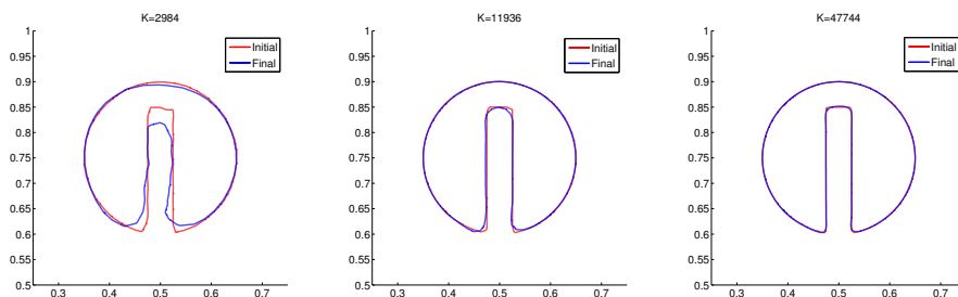
Figure 7.6: Zalesak's slotted disc at t = T , for the MCLS field, using n = 1 .
