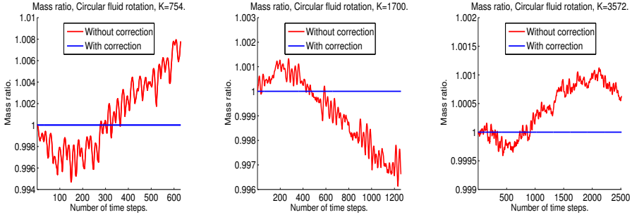
Figure 4.15: Time history of mass error for the circular fluid rotation case.
