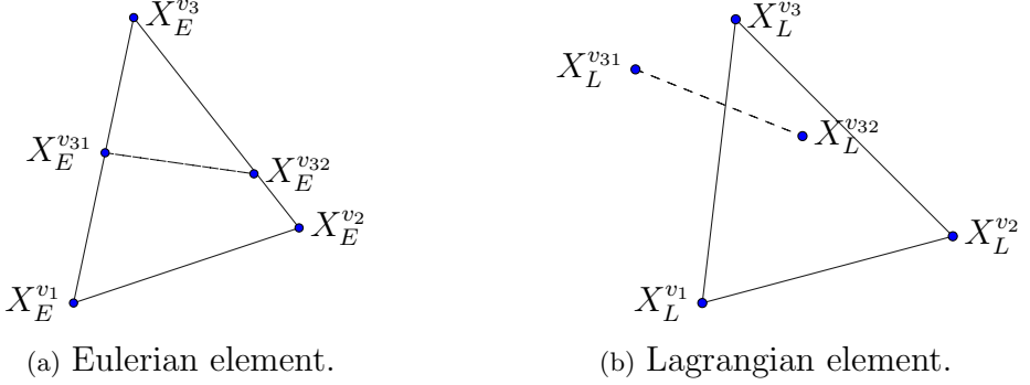
Figure 4.12: The position of the interface in a mixed cell in the Lagrangian mesh is based on the advection of the extremities of the interface in the corresponding mixed cell in the Eulerian mesh.
