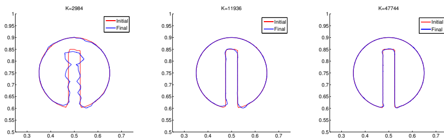
Figure 7.5: Zalesak's slotted disc at t = T , for the LS field, using n = 1 .
