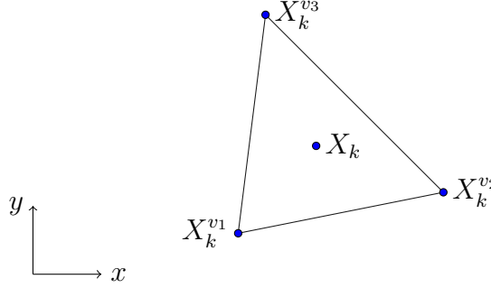
Figure 2.2: Control volume ( \Omega_k ).
