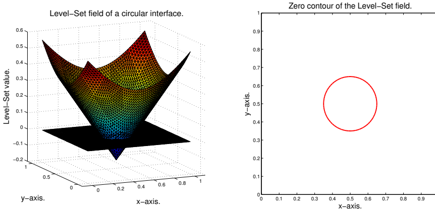
Figure 2.1: The level-set field and the corresponding zero-level contour of the interface.
