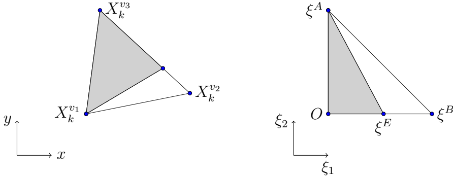
Figure 4.4: Interface passing through vertex (X_k^{v1}) .
