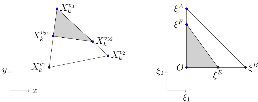
Figure 4.3: Case-1: Triangular domain of interest, where the vertex \mathbf{X}_k^{v3} is mapped to the origin.
