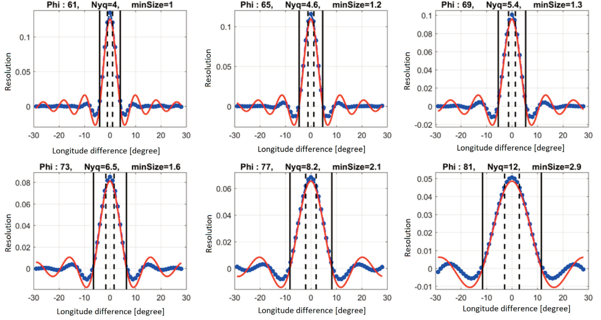
Figure 15. Fitted sinc pattern at six different latitudes (ordered from south to north) for 2-degree solution.
