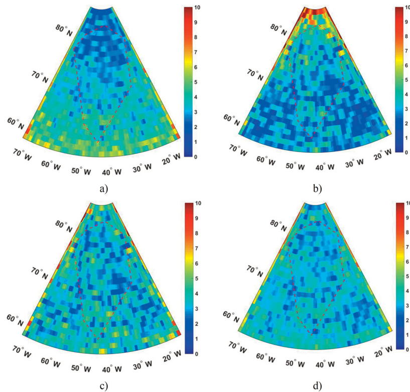
Figure 9. The empirical standard deviations ( \text{kg/m}^2 ) of 1-degree solution obtained from weight matrix for Case 2 (342 arcs and 1-degree grid) with weights P_0 (a), P_1 (b), P_2 (c) and P_3 (d).
