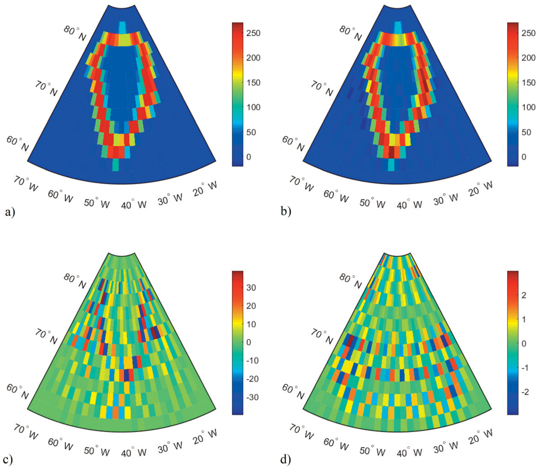
Figure 11. True values of surface density changes of Greenland (a: up-left), retrieved from inversion of x \leftarrow Rx where x = U_1 U_1^T x + U_2 U_2^T x is inverted to x = U_1 U_1^T x + \frac{\lambda}{\alpha} U_2 U_2^T x due to regularization; recovered values (b: up-right), unrecovered values (c: down-left), and distorted unrecovered values (d: down-right).
