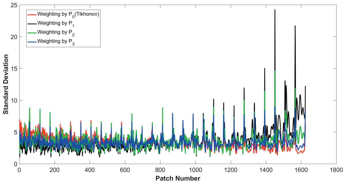
Figure 8. The Empirical standard deviations ( \text{kg/m}^2 ) of estimated surface density changes regularized by four weight matrices for Case 2 (342 arcs and 1-degree grid).
