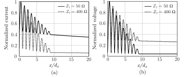
Fig. 9. (a) Normalized current in a dipole loaded periodically with Z_l = 50 \Omega and Z_l = 400 \Omega ; (b) normalized voltage in a slot periodic with periodic shunt loads Z_l = 50 \Omega and Z_l = 400 \Omega . Both the dipole and the slot have width w_d = w_s = \lambda/30 and are loaded with 9 resistors located at periodic distance d_x = 0.5\lambda .
