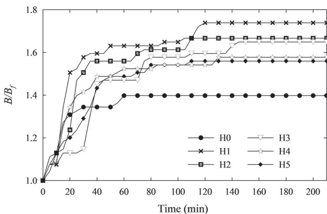
Figure 11 Dimensionless channel width evolution as a function of time for all the considered the hydrographs on the sediment sample S4
