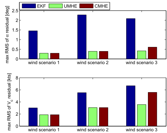
Fig. 3. Comparison of robustness to disturbances of the EKF-FTE, UMHE-FTE, and CMHE-FTE in different wind scenarios without faults: maximum rms of the residuals for AOA and VCAS with p_w = 0.01 and q_w = 0.1 .
