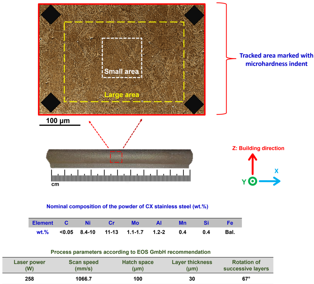
Fig. 1—An image of the rod-shaped CX SS sample printed horizontally, and the X-Z plane cut from the sample marked with the microhardness indents for tracking microstructure. The small and large area for microstructural tracking using quasi in situ EBSD as well as the process parameters used for its fabrication are also shown.
