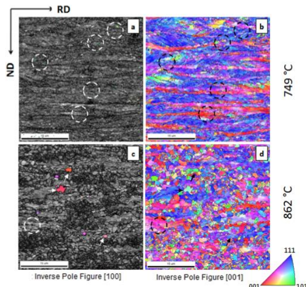
Figure 12. Microstructure of samples heated at 1500°C/s to 749°C (a,b), and to 862°C (c,d). The microstructure consists of a mixture of ferrite and martensite. Arrows indicate grains oriented close to the Goss \{110\}\langle 001 \rangle (c,d), and circles the rotated Goss \{110\}\langle 011 \rangle (a,b) components. (a,c) correspond to IQ maps in which the recrystallized grains of ferrite are highlighted by a [100] RD Inverse Pole Figure (IPF) map. (b,d) are [001] ND IPF maps [9].
