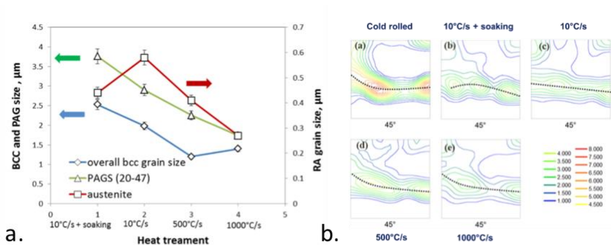
Figure 14 (a) Dependence of the average grain size from the heating rate and the isothermal soaking; (b) ODFs showing the texture evolution as a function of the heating rate and soaking time. The dotted line displays typical curvature of the ND fibres observed in cold rolled and recrystallized steels.
