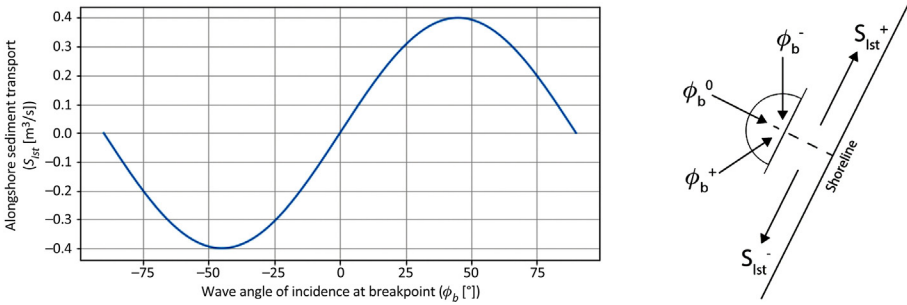
Figure 9.8 Left panel shows schematic representation of S-\phi_b curve for an arbitrary wave height at breakpoint. Right panel shows schematic representation of different wave angles leading to different longshore sediment transport directions.
