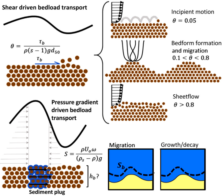
Figure 9.6 Mechanisms of bedload sediment transport. Shear (top) versus pressure gradient-induced (bottom left) sediment transport. Note, shear-driven transport mechanics (incipient motion, bedform formation/migration and sheet flow) are relevant to both wave- and current-driven flows, whereas pressure gradient-driven transport is most relevant to wave-driven flow. Mechanism for bedform migration and growth (bottom right). When the transport is in phase with the bedform shape, the bedform will migrate; when out of phase, the bedform will grow (phase offset to the left of bedform crest—shown) or decay (phase offset to the right of bedform crest—not shown).
