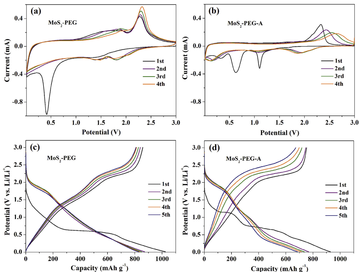
Fig. 7. Cyclic voltammograms of MoS 2 -PEG (a) and MoS 2 -PEG-A (b) at a scan rate of 0.1 mV s −1 . The charging-discharging curves of MoS 2 -PEG (c) and MoS 2 -PEG-A (d) at a current density of 0.1 A g −1 .
