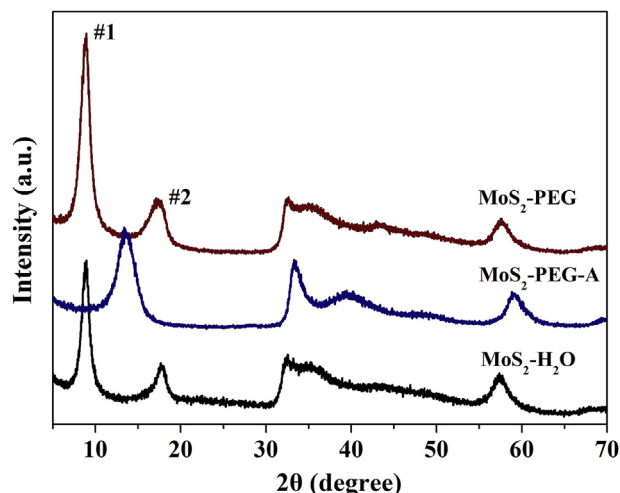
Fig. 1. XRD profiles of \text{MoS}_2\text{-PEG} before and after annealing at 550 °C and \text{MoS}_2\text{-H}_2\text{O} .
