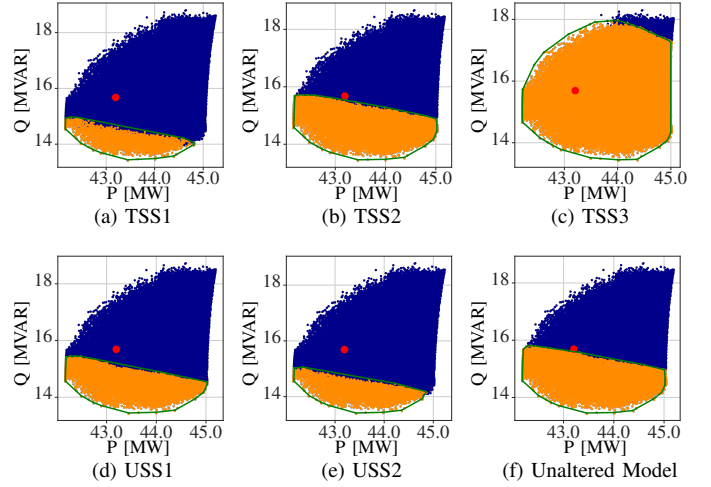
Fig. 4: Flexibility areas for 6 scenarios with similar observable network component values but different unobservable network component values. Feasible flexibility samples (orange), infeasible flexibility samples (blue), initial operating point (red), and convex hull area of feasible samples (green).
