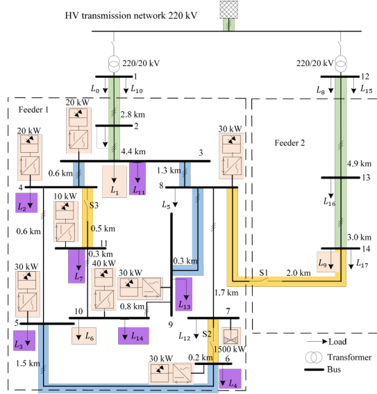
Fig. 3: CIGRE MV DN with solar photovoltaic and Wind DER with modifications. Observable lines (green). FSPs (orange). TSS altered lines (blue) and switches (yellow). USS/TSS altered loads (purple).
