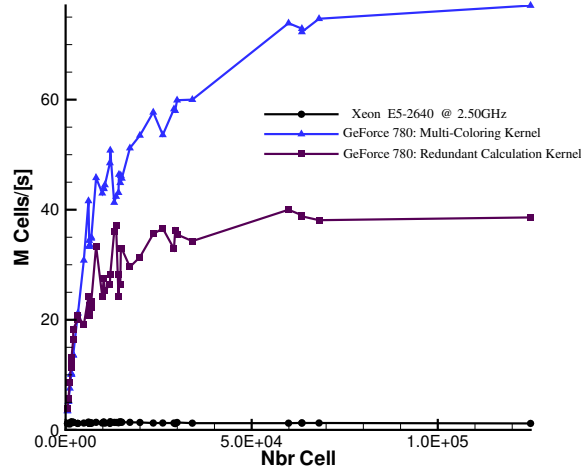
Figure 4: Performance in terms of updated cells per second for one inviscid flux calculation on a single CPU compared to multi-coloring based kernel and redundant calculation on GeForce 780 for a RANS simulation of 2D flow on a supersonic compressor cascade
