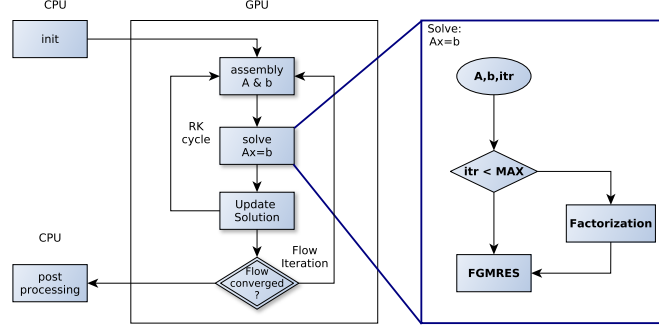
Figure 8: Flow Solver algorithm showing the full GPU assembly and linear solver with on-demand factorization
