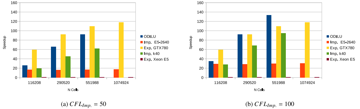
Figure 12: Speedup of all solvers with reference to the explicit solver on E5-2640 for two different CFL numbers for the implicit solver and the same CFL number for the explicit solvers ( CFL_{Exp.} = 2.5 ).
