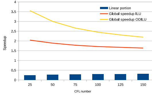
Figure 13: Plot of the effect of the CFL increase on the portion of the linear solver on CPU and the global speedup both with full ILU update and on-demand update (OD-ILU)
