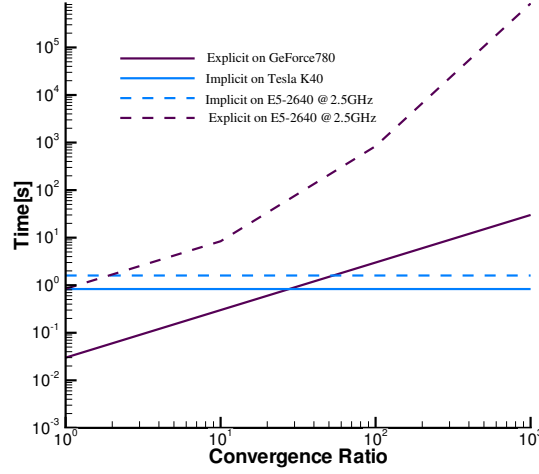
Figure 6: Execution time of implicit solver for one flow iteration and explicit solver for equivalent flow iterations both on the CPU and the GPU as a function of the convergence ratio for a turbine nozzle guide Vane(Blade definition from [42])
