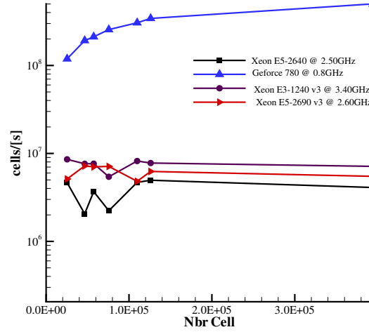
Figure 5: Performance in terms of updated cells per second for one Runge-Kutta stage on a Geforce 780 compared to 3 other single CPUs for a RANS simulation of 2D flow on a supersonic compressor cascade
