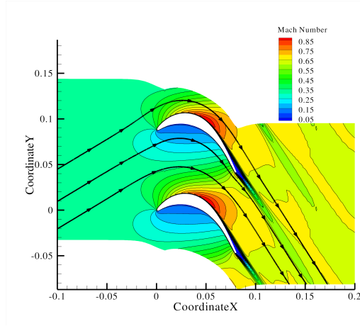
Figure 9: Mach number contours around the t106c nozzle guide vane
