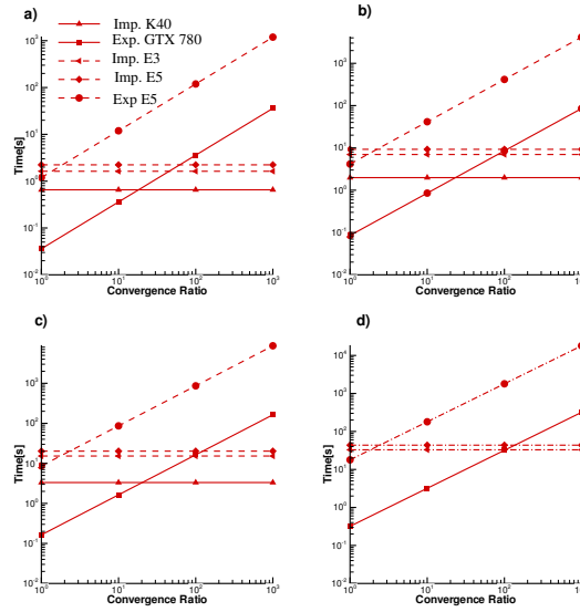
Figure 11: case t106c: Execution time of implicit solver for one flow iteration and explicit solver for equivalent flow iterations both on the CPU(dashes line) and the GPU (full line) as a function of the convergence ratio for increasing mesh resolution (a: smallest mesh, d: largest mesh)
