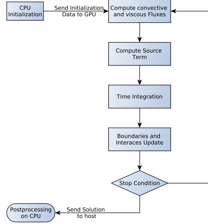
Figure 7: The Solver computes firsts inviscid and viscous Residuals and source term. Second the time integration takes places and finally boundaries and mesh interfaces are updated
