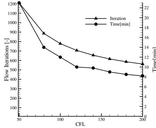
Figure 1: Saturation of the iterations number with the increase of CFL number (case: turbine t106c [8])
