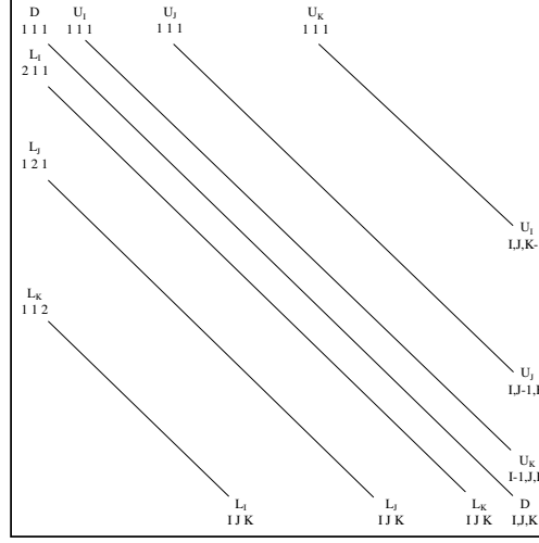
Figure 2: Structure of the system matrix showing 7 diagonals filled with block matrix of N_v * N_v with N_v the number of flow variables. I, J and K are the number of cells in the first, second and third direction respectively.
