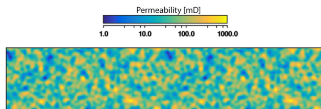
Fig. 21 Case 2: permeability realization with dimensionless correlation length \lambda=0.01 and V_{dp}=0.63
