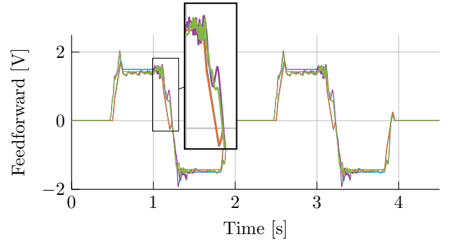
Fig. 7. Feedforward signals for r_1 produced by F(q) (—) and by the GP-based method (—), and for r_2 by F(q) (—) and by the GP-based method (—). The GP leads to a more complex signal, possibly to compensate for position-dependent static friction.
