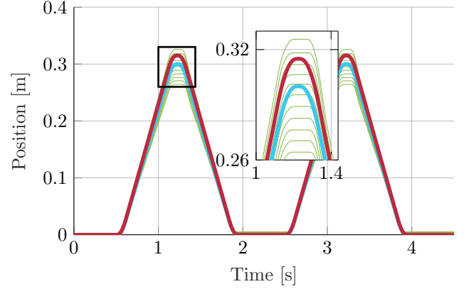
Fig. 6. References r_1 (—) and r_2 (—) and observed outputs y_i (—) from 11 closed-loop experiments using signals \tilde{r}_i .
