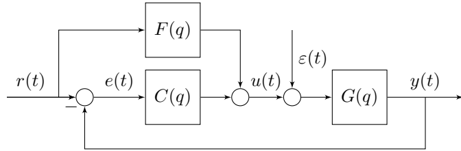
Fig. 2. Motion control architecture.
