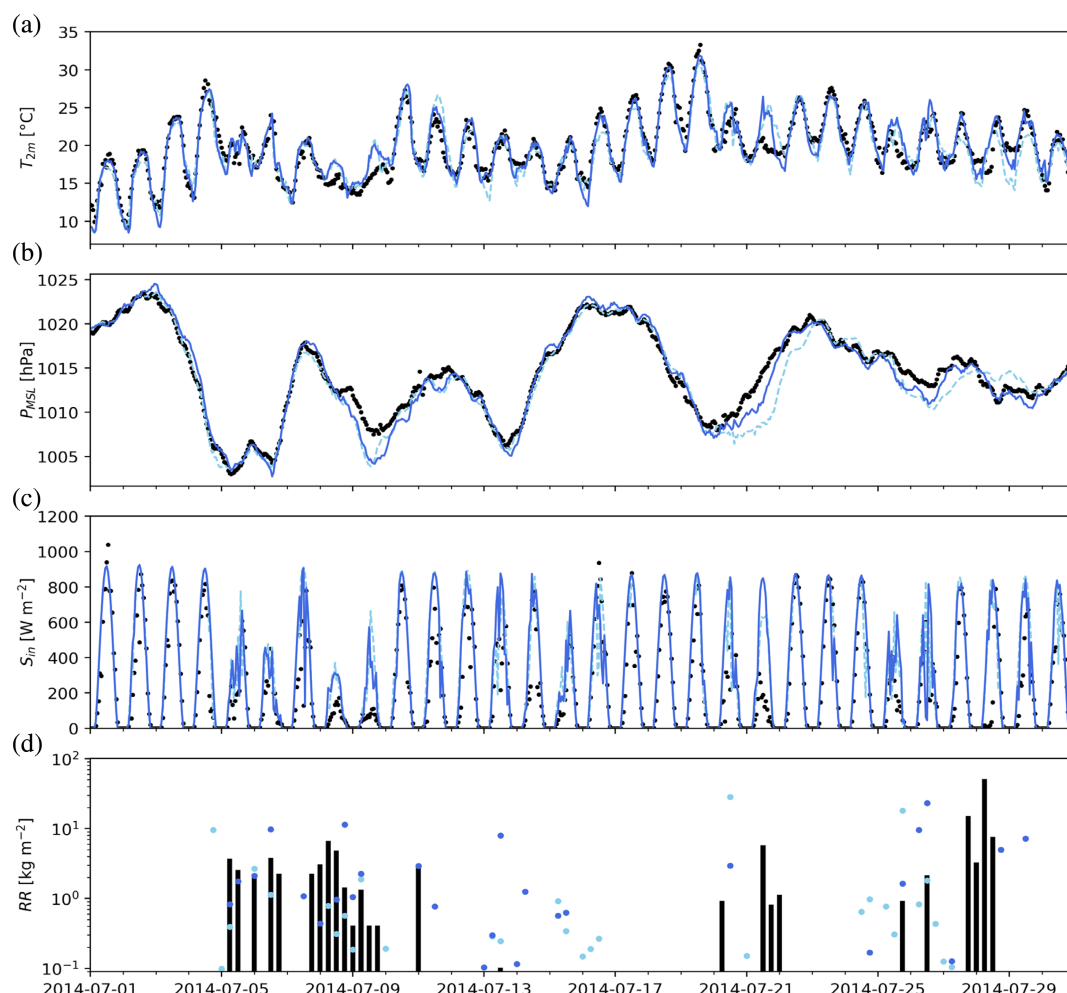
FIGURE 4 Time series of modelled and observed (a) 2-m temperature, (b) mean sea-level pressure, (c) downwelling solar radiation, and (d) precipitation at Schiphol airport weather station (52.301°N, 4.774°E, WMO code 6240) for July 2014. The black dots and bars indicate the observations, the dark blue solid lines and dots the WMO stations data assimilation (WMO-DA) run and the light blue dashed lines and dots the no data assimilation (NO-DA) run [Colour figure can be viewed at wileyonlinelibrary.com ]
