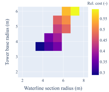
Figure 20: Material cost normalised to 0 – 1. Only feasible designs are shown.
