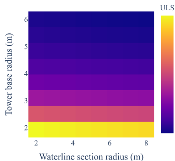
Figure 13: Tower base section strength utilisation.
