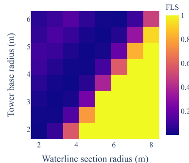
Figure 14: Tower base fatigue damage.
