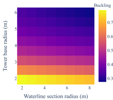
Figure 18: Tower buckling.
