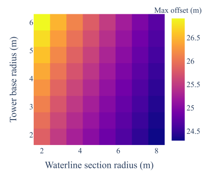
Figure 9: Maximum offset.
