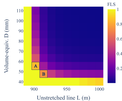
Figure 6: Mooring line fatigue damage.
