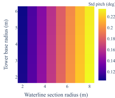
Figure 8: Dynamic pitch displacement.
