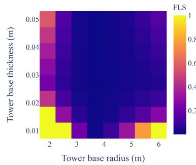
Figure 16: Tower base fatigue damage – the effect of wall thickness.
