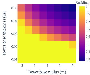
Figure 19: Tower buckling – the effect of wall thickness.
