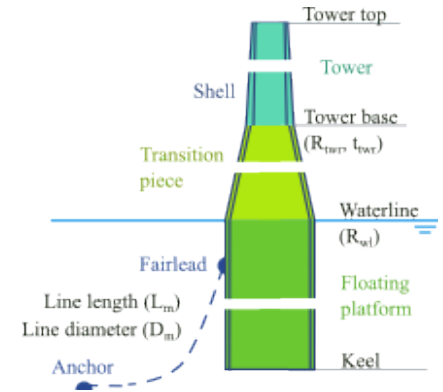
Figure 4: Design variables.
