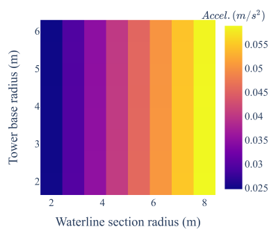
Figure 10: Tower top resultant acceleration in rated conditions.
