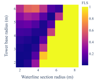
Figure 12: Waterline section fatigue damage.
