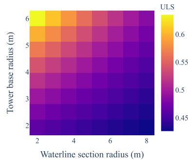
Figure 11: Waterline section strength utilisation.
