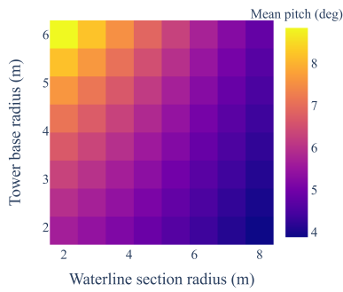
Figure 7: Mean pitch displacement.
