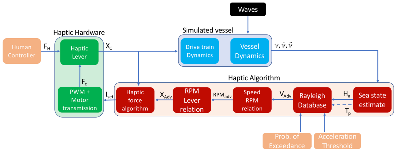
Figure 5: A block diagram showing the human controller acting on the haptic hardware, which controls the simulated vessel and the haptic algorithm used to provide a haptic speed advice.
