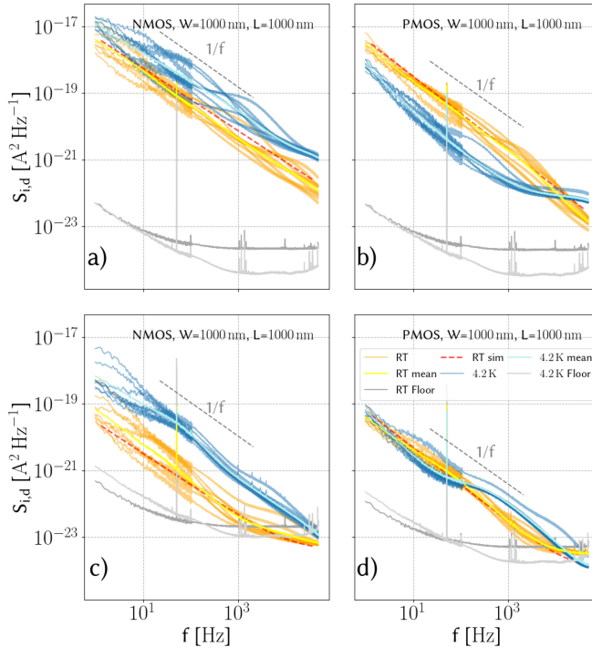
FIGURE 3. Noise spectra for NMOS (a, c) and PMOS (b, d) with W \times L = 1\mu\text{m} \times 1\mu\text{m} at V_{gs}=1.1\text{V} and V_{ds}=1.1\text{V} (a,b) and V_{ds}=50\text{mV} (c,d), respectively. 8 devices at the same bias points are shown.
