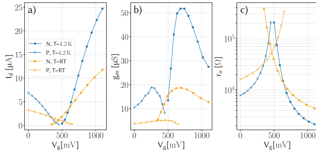
FIGURE 2. Example N/PMOS ( 1\mu\text{m} \times 1\mu\text{m} ) DC-characteristics at V_{ds}=50\text{mV} : a) drain current I_d , b) transconductance g_m , c) output resistance r_o .
