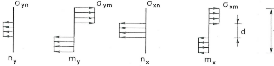
Fig. 6: Plate bending moments and plate normal forces with optimal stress distribution in the tube wall
