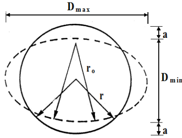
Fig. 10: Definition of ovalisation, radius r_o and critical curvature in an ovalised cross section
