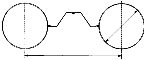
Fig. 1: Schematic and photo of a combined wall of tubes and infill sheeting, also called CombiWall; the infill sheeting is connected to the tubes with welded slots
