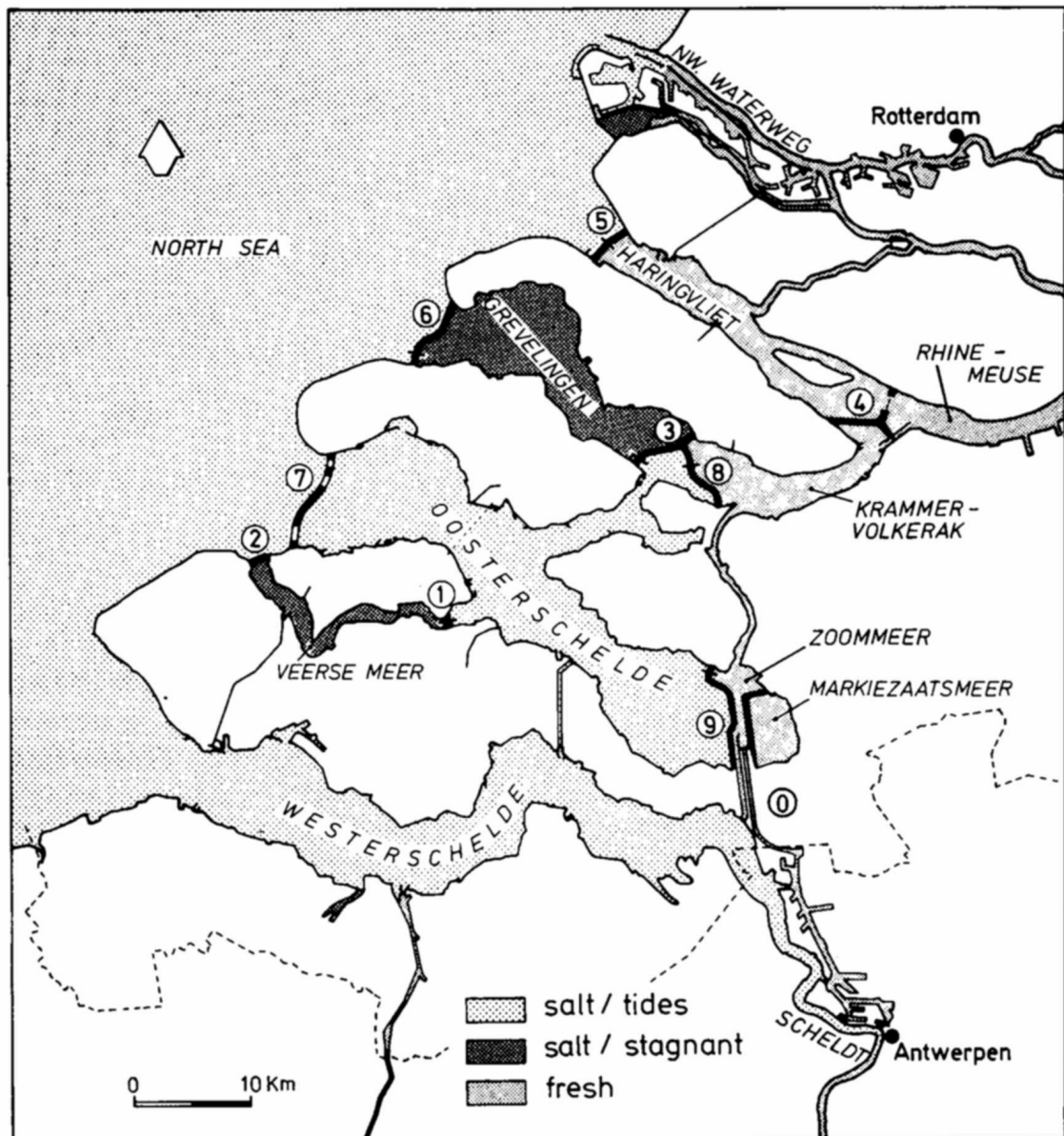
Figure 3.3. Overview of the present-day Delta Region, i.e. after completion of the Delta Plan (Nienhuis & Smaal, 1997). 0 = Kreekrakdam (1867), 1 = Zandkreekdams (1960), 2 = Veersegatdam (1961), 3 = Grevelingendam (1964), 4 = Volkerakdam (1969), 5 = Haringvlietdam (1970), 6 = Brouwersdam (1971), 7 = Storm-surge barrier (1986), 8 = Philipsdam (1987), 9 = Oesterdam (1986). Markiezaatsmeer has been disconnected from Zoommeer in 1983.
