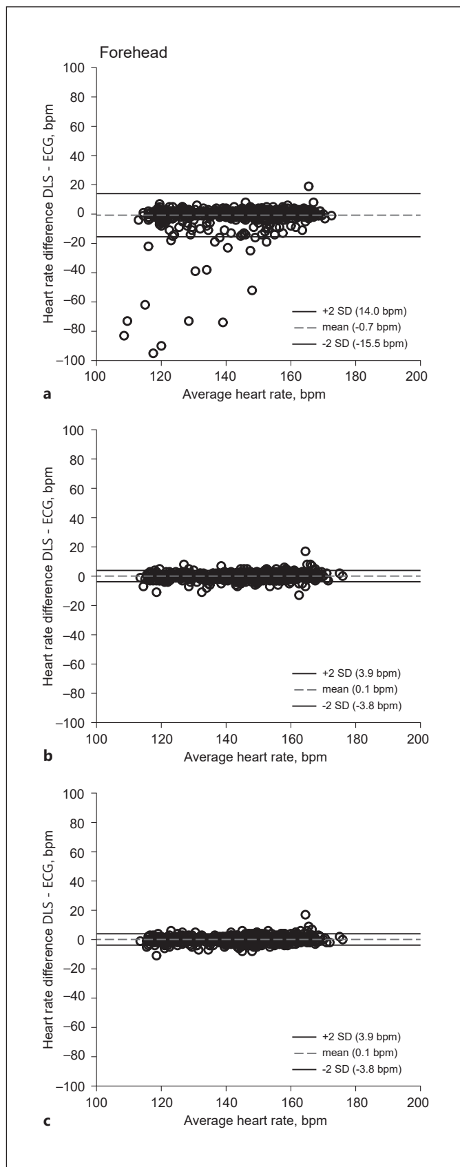
Fig. 4. Bland-Altman plots (A-B plot) of the heart rate (HR) difference against the average HR during measurements performed at the forehead. a Agreement between DLS and ECG HR of data pairs with a DLS SNR above the calculated cut-off value (1.66). b Agreement between the standard of care POX (POX-S) and ECG HR. c Agreement between the additional POX (POX-A) and ECG HR.
