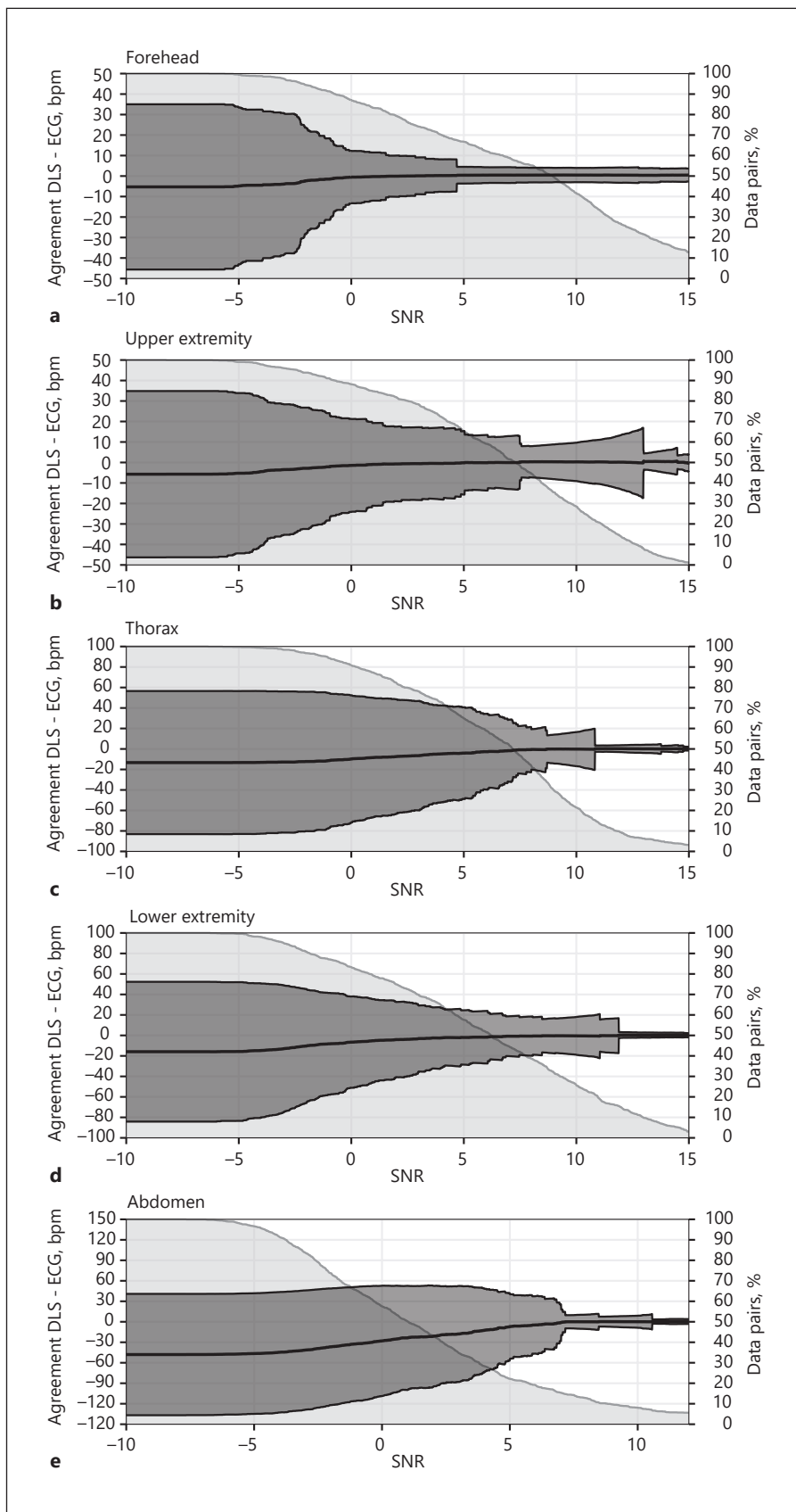
Fig. 3. Agreement (A-B plot) between heart rate measurements obtained with the mDLS™ sensor and ECG, plotted for every measured DLS SNR value at the forehead (a), an upper extremity (b), the thorax (c), a lower extremity (d), and the abdomen (e). Agreement is presented as bias with upper and lower limits of agreement (dark grey). The percentage of remaining data pairs (DLS-ECG) used for the Bland-Altman analyses are illustrated against the SNR (light grey).
