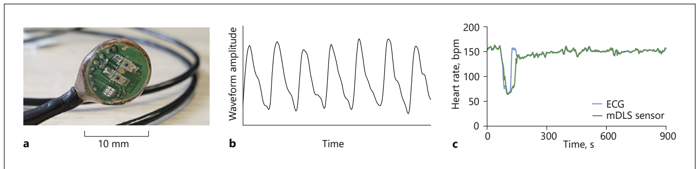
Fig. 1. a mDLS™ sensor. b Waveform example of the DLS measurement, illustrating the sphygmogram in an infant. c An example of the measured heart rate trend of ECG and DLS at the abdomen.
