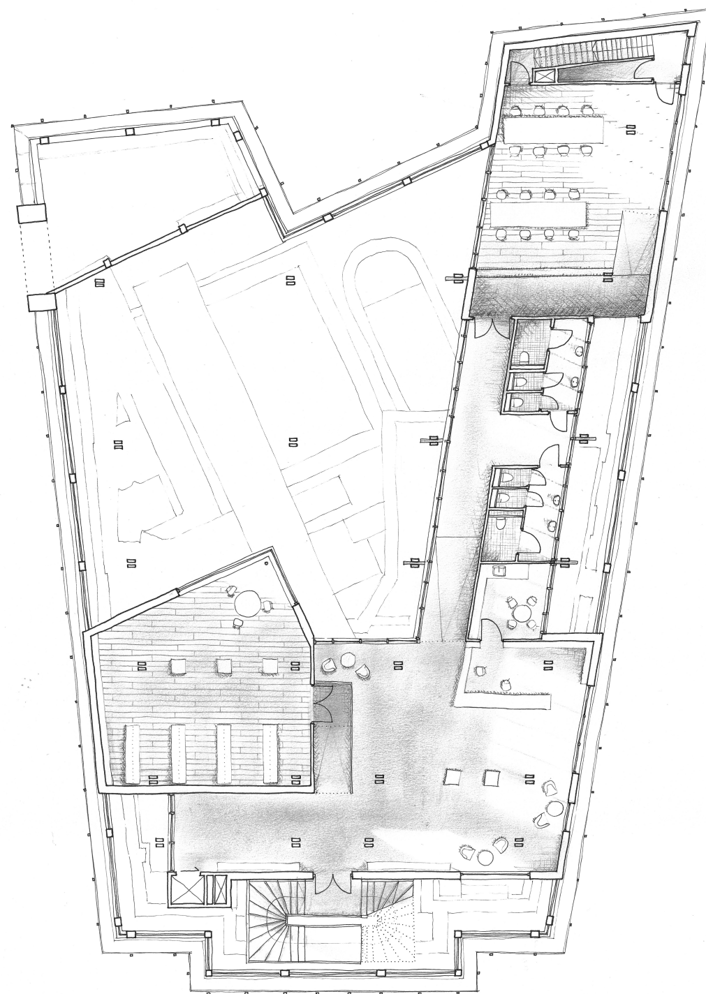
floor plan, first floor 1:250 (original 1:100)
