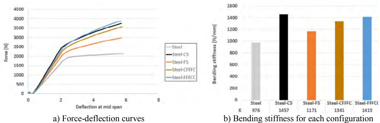
Figure 4. Force-deflection simulation results.
