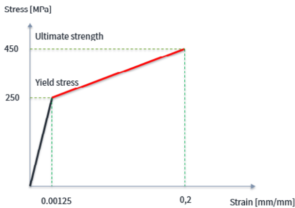
Figure 2. Stress-Strain bilinear law for A36 Steel.
