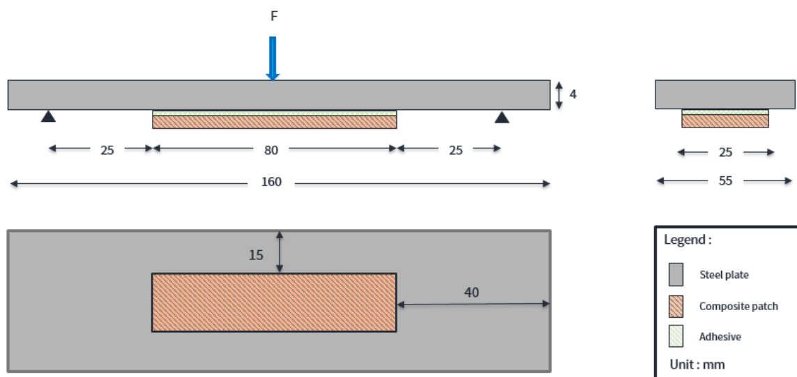
Figure 1. Schematic of a composite-strengthened steel plate.
