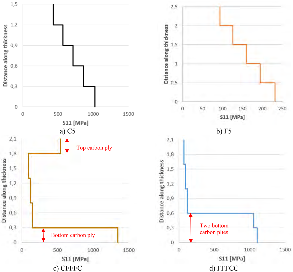
Figure 5. Distance along the thickness of the composite patches vs longitudinal stresses at mid-span
