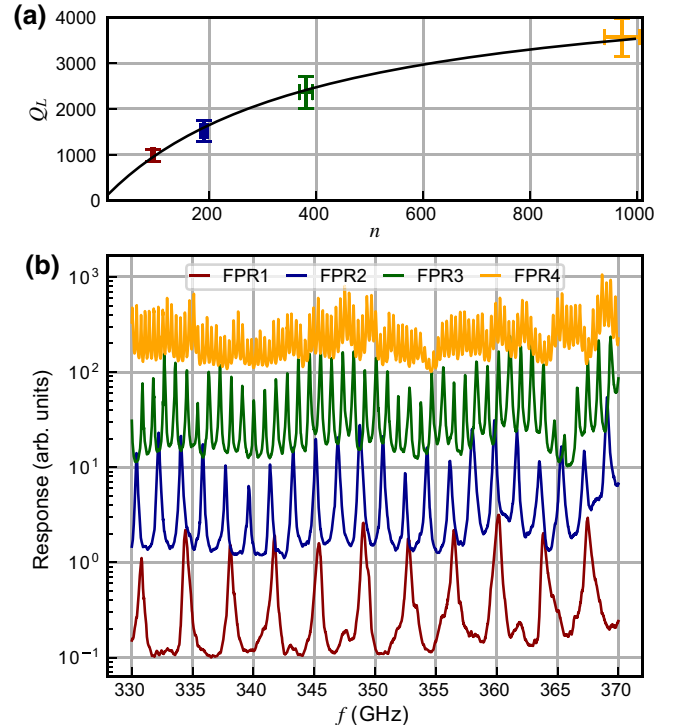
FIG. 3. (a) Averaged loaded quality factor Q_L as a function of average mode number in the four FPRs. The fit using Eq. (1) is shown by the black line. (b) Measured spectra of the FPRs, offset along the y axis for better comparison. Line colors correspond to the markers in (a).
