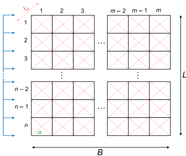
Fig. 5. Schematic representation of a diaphragm simulated with macro-elements.
